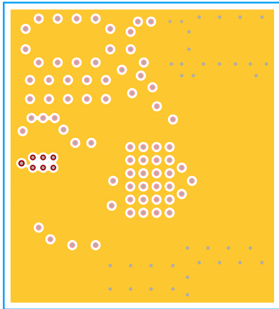
Figure 8. Layer 3
