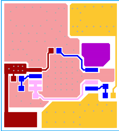
Figure 6. Top Layer
