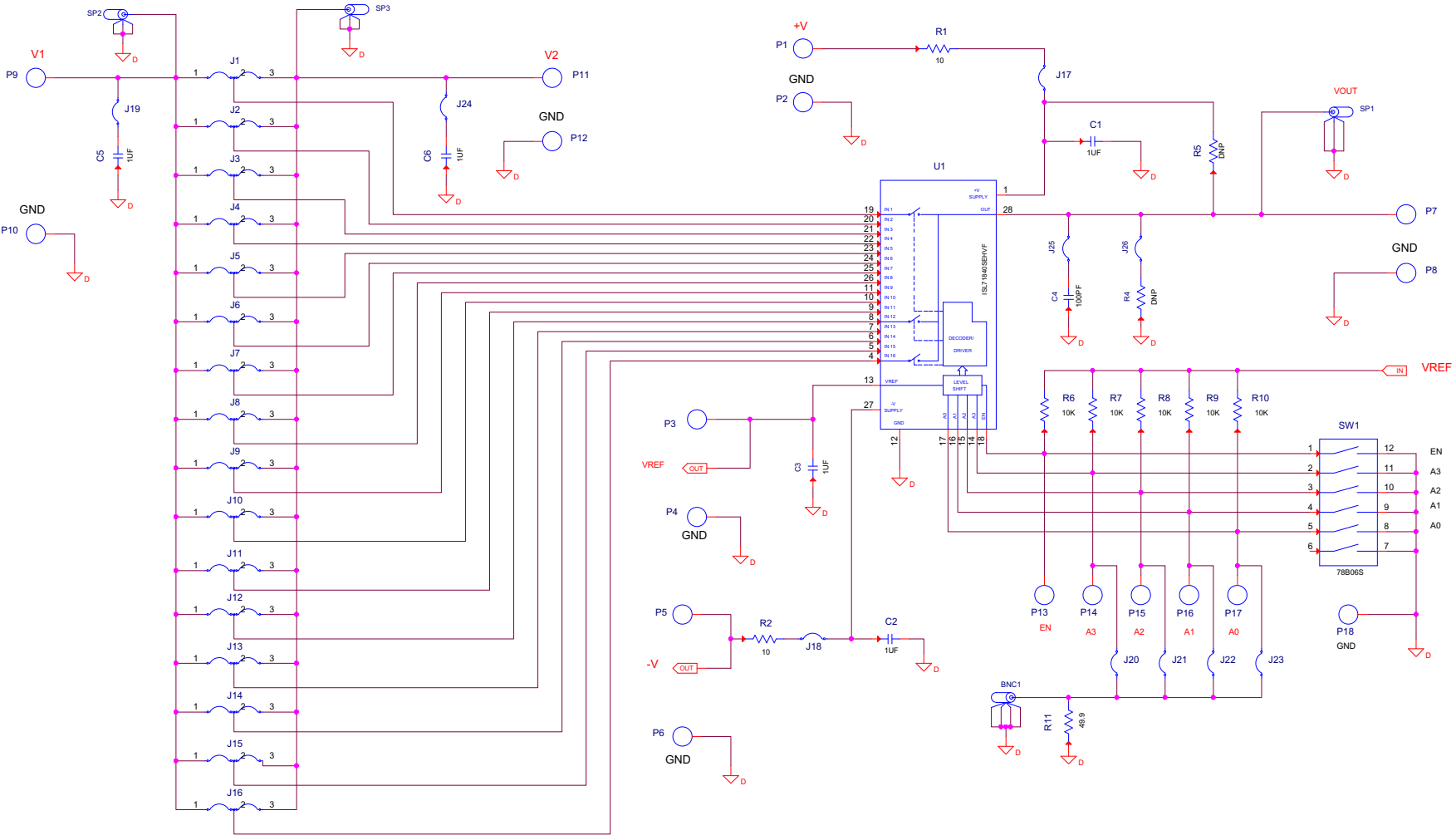
FIGURE 4. ISL71840SEHEV1Z SCHEMATIC
