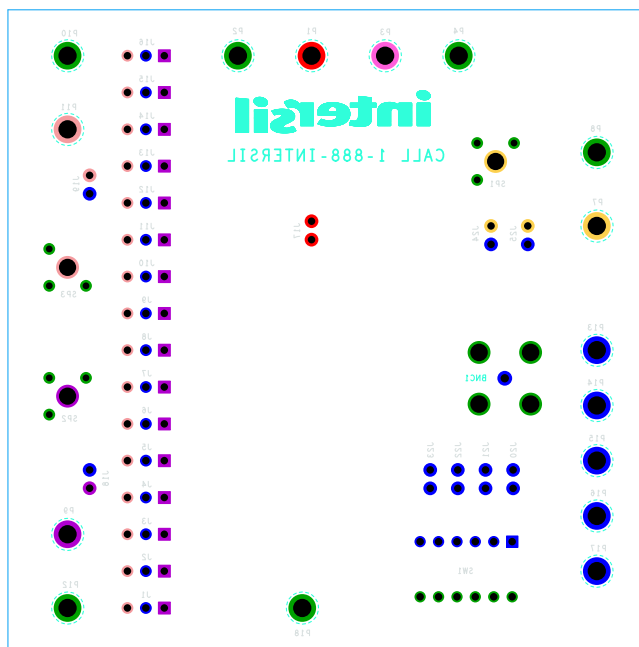
FIGURE 10. SILKSCREEN BOTTOM
