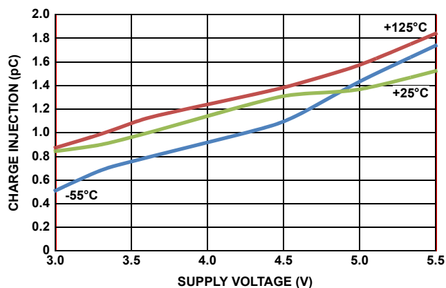
FIGURE 16. CHARGE INJECTION
