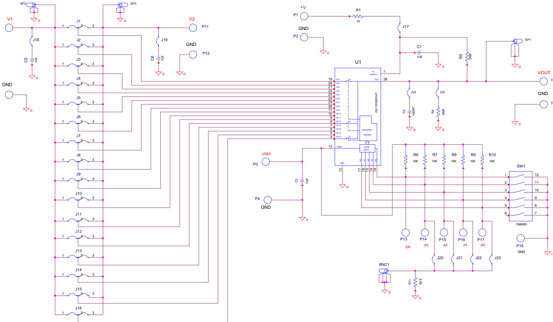
FIGURE 4. ISL71830SEHEV1Z SCHEMATIC
