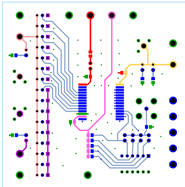
FIGURE 6. TOP LAYER
