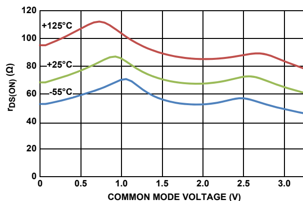
FIGURE 12. r_{DS(ON)} vs COMMON MODE VOLTAGE ( V_S = +3.3V )
