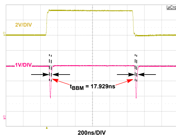
FIGURE 14. BREAK-BEFORE-MAKE DELAY
