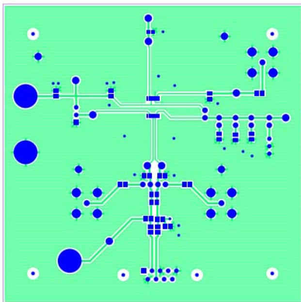
Figure 5.3 Top Layer
