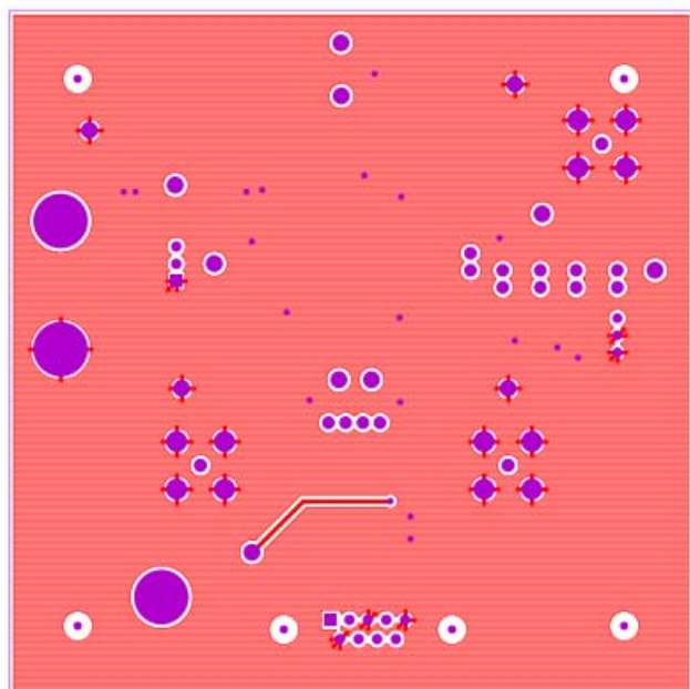
Figure 5.4 Bottom Layer
