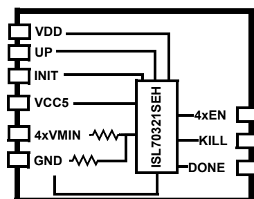
Figure 1. Block Diagram
