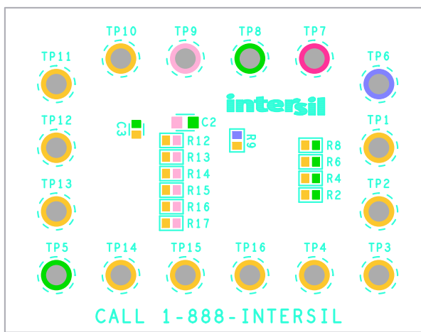
Figure 14. Bottom Silkscreen
