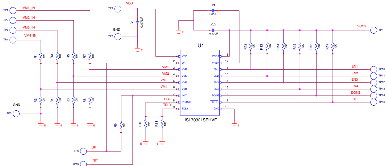
Figure 10. ISL70321SEHDEMO1Z Schematic
