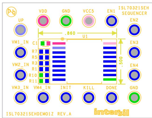
Figure 11. Top Silkscreen
