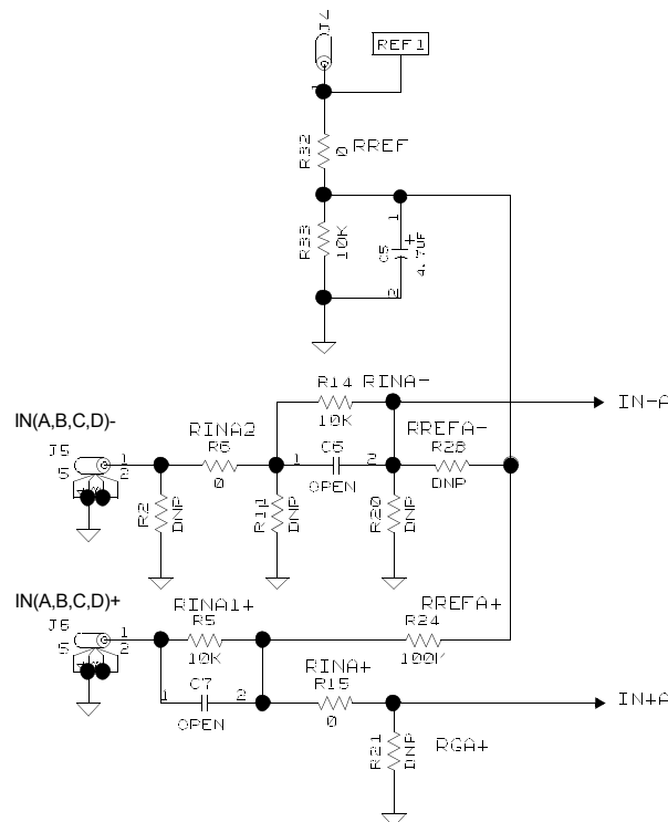
FIGURE 3. COMPONENT-SELECTABLE OPTIONS
