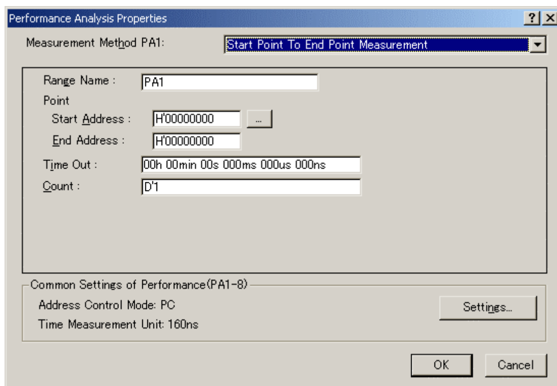
図 5-62 Start Point To End Point Measurement 設定
