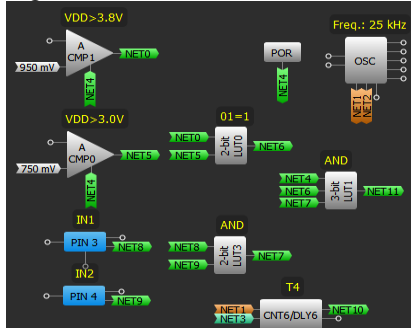
Figure 3-15. Labeled connections
