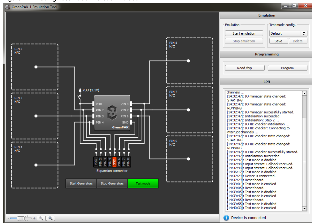
Figure 7-42. Using Test Mode Without Emulation
