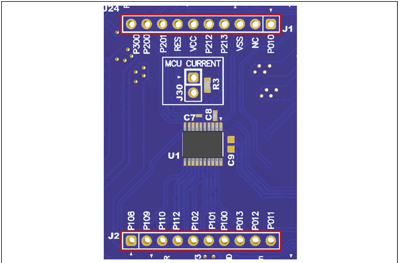
図 19 Native Pin Access (Breakout Pin Header J1, J2) (表面)
