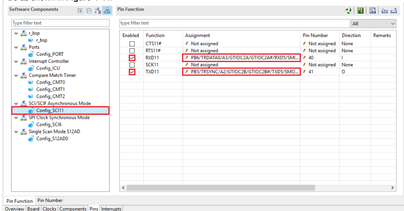
Figure 4-44 Configure pin assignment - Config_SCI11
