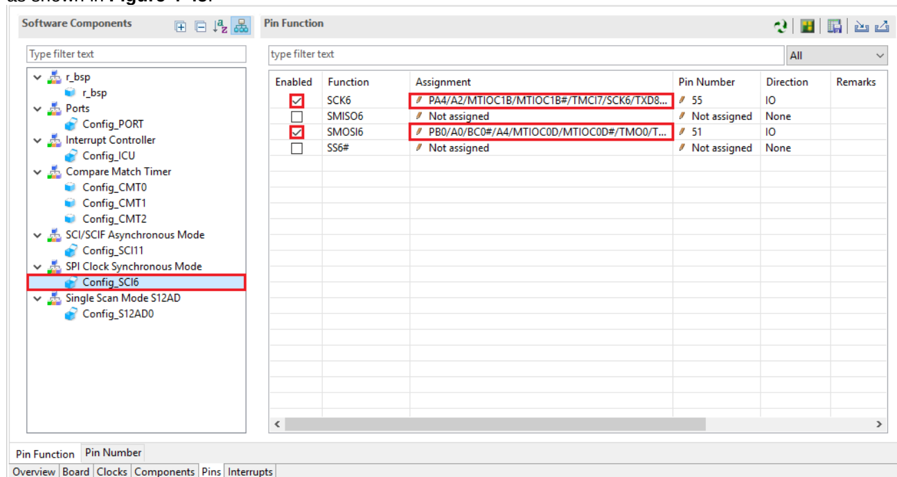
Figure 4-45 Configure pin assignment - Config_SCI6
