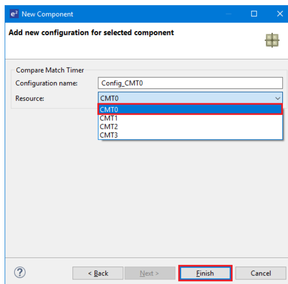
Figure 4-10 Select Resource - CMT0
