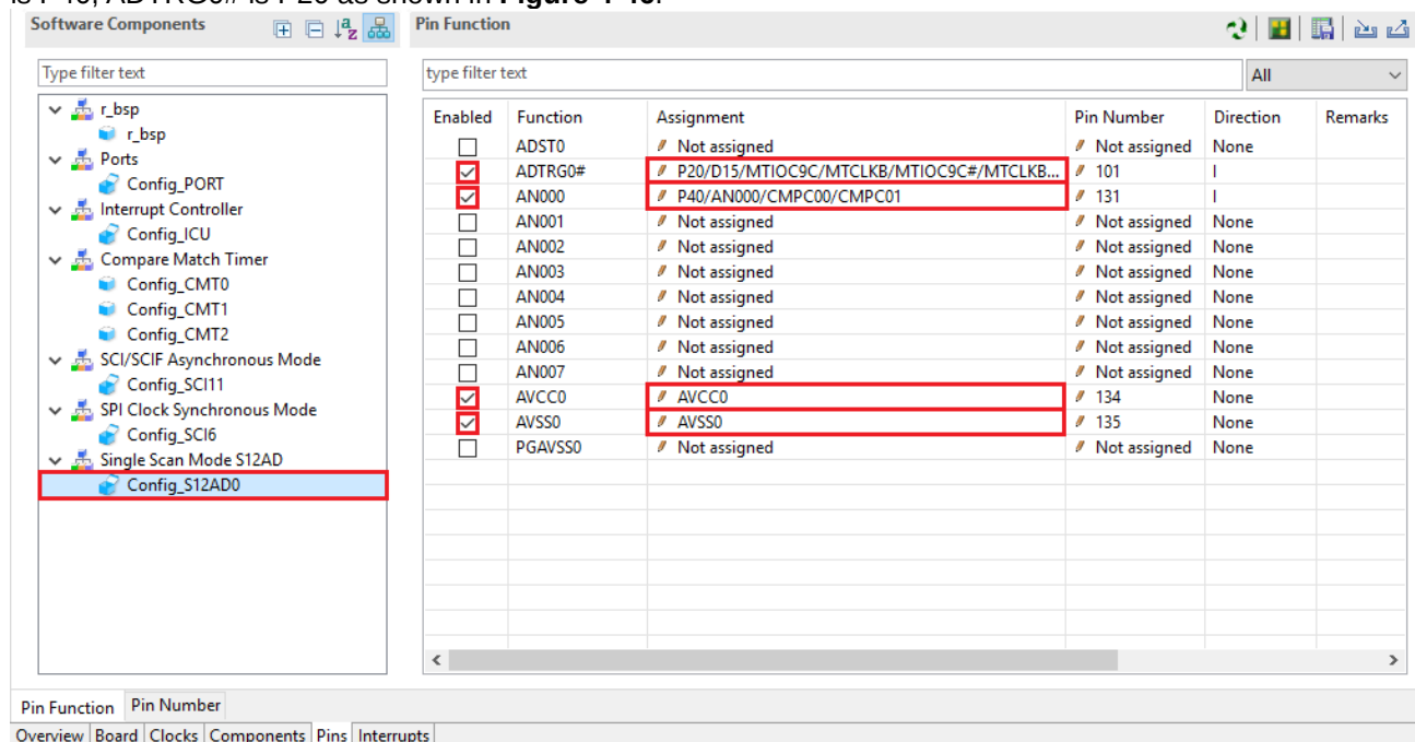
Figure 4-46 Configure pin assignment - Config_S12AD0
