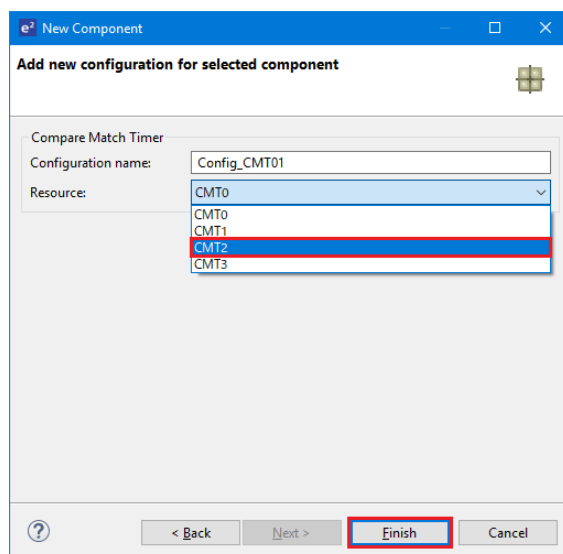
Figure 4-14 Select Resource – CMT2
