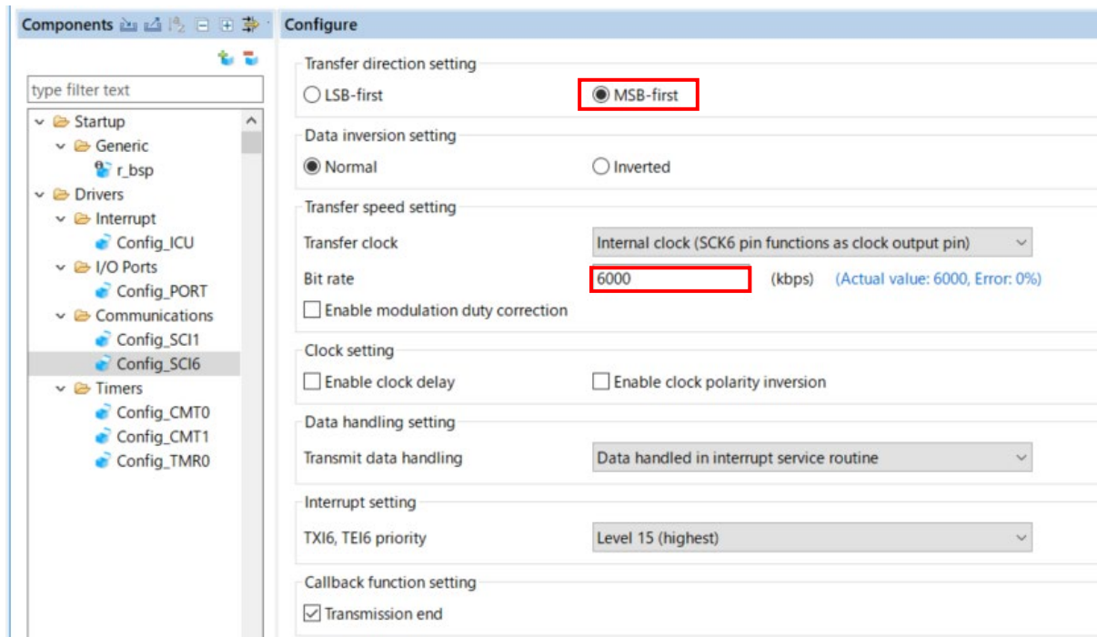
Figure 4-41 Config_SCI6 setting
