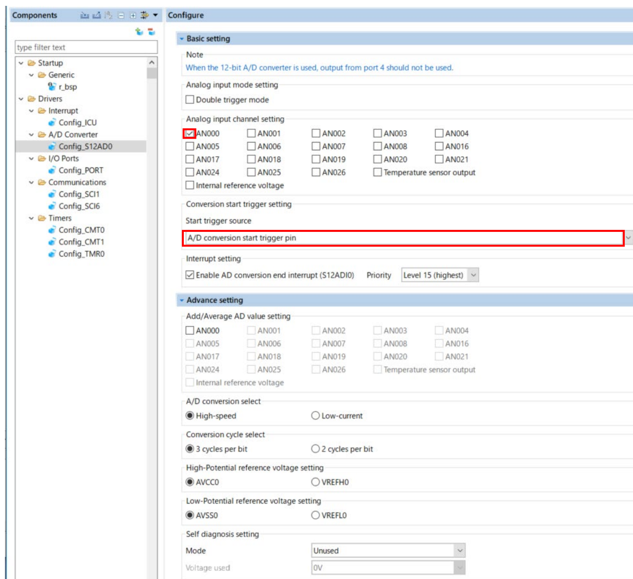
Figure 4-44 Config_S12AD0 setting (1)
