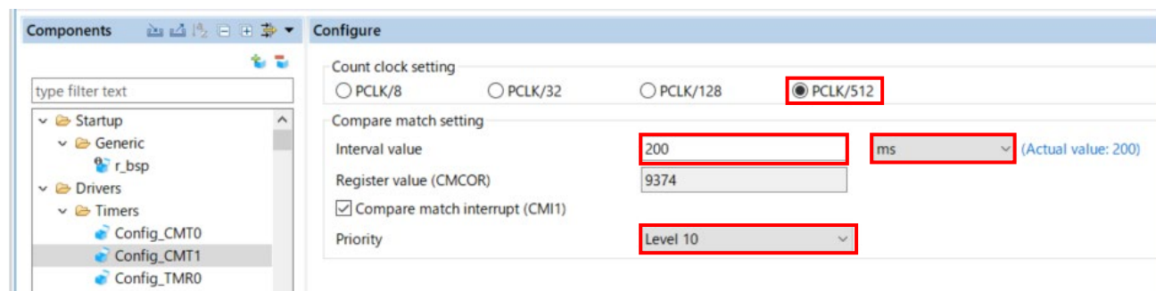
Figure 4-20 Config_CMT1 setting
