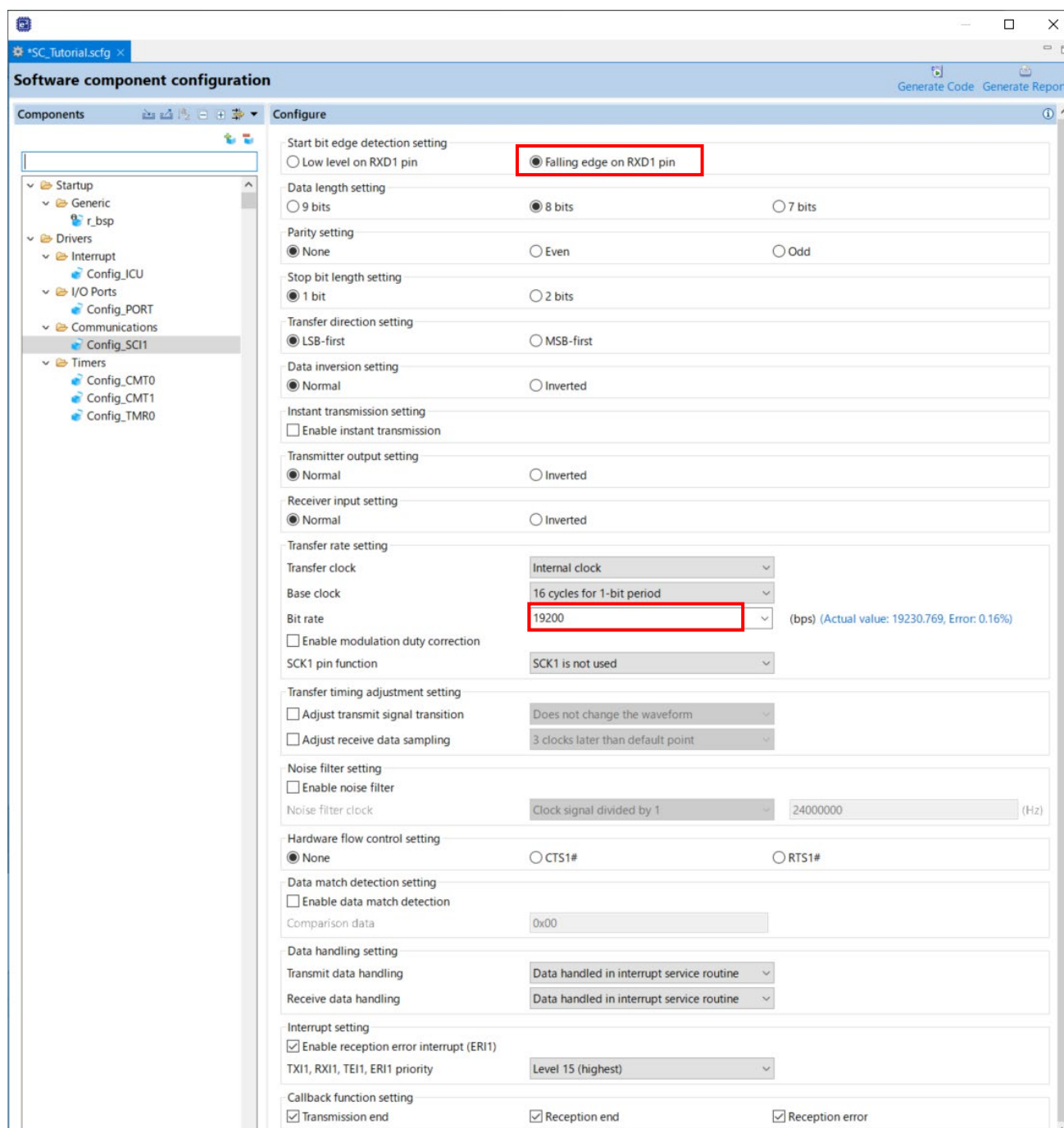
Figure 4-36 Config_SCI1 setting
