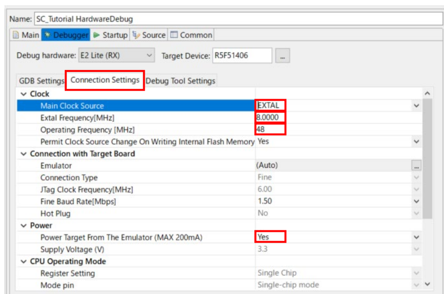
Figure 6-2 Connection Settings
