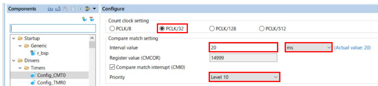
Figure 4-17 Config_CMT0 setting
