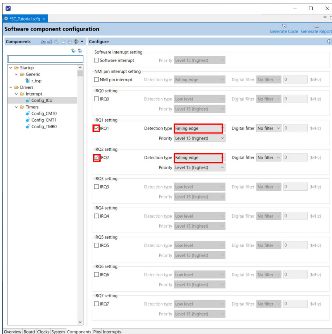
Figure 4-23 Config_ICU setting
