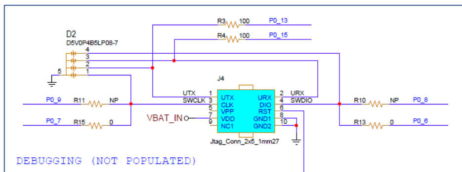
Figure 11. The debugging header, J4
