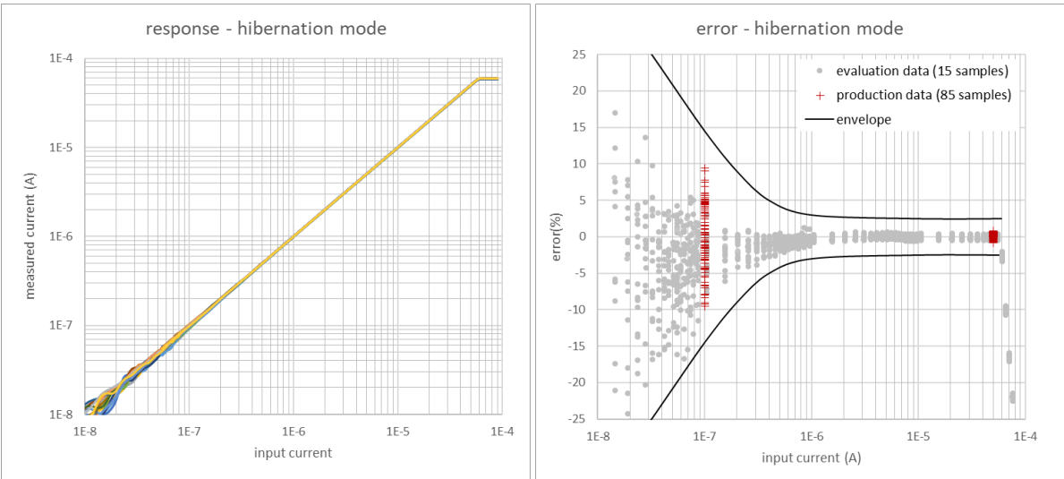
Figure 38. Hibernation mode (100 nA to 60 \mu A at 3.3 V) data after offset calibration
