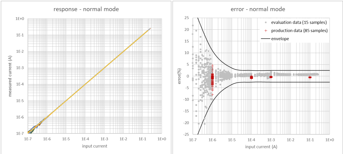
Figure 37. Normal mode (1 \mu A to 640 mA at 3.3 V) data after offset calibration
