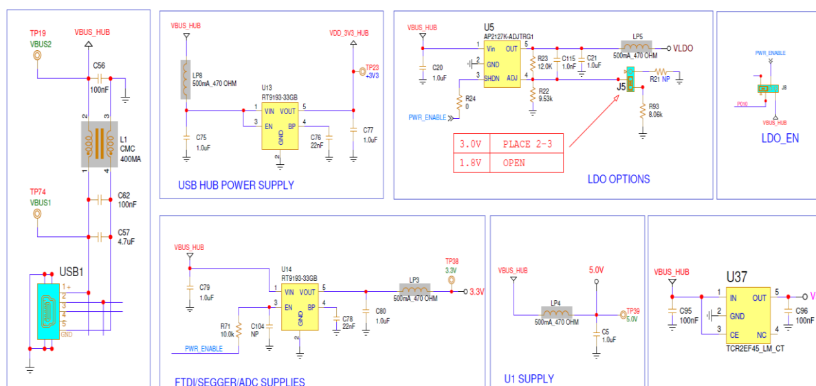
Figure 29. DA1459x Pro-motherboard power section
