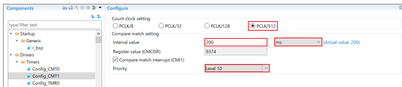
Figure 4-19 Config_CMT1 setting
