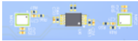
Figure 19. MEMS MICs
