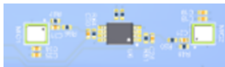
Figure 15. MEMS MICs
