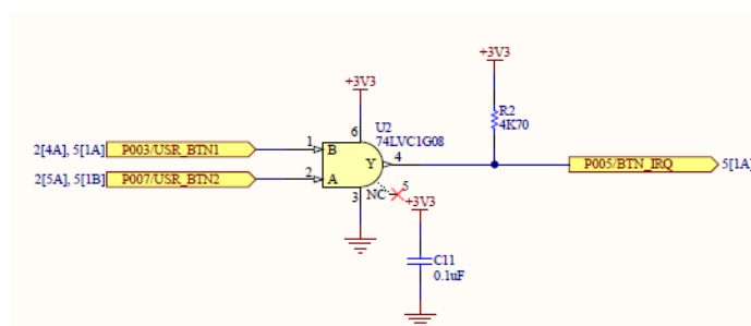
Figure 13: S2 + S3 User Switches
