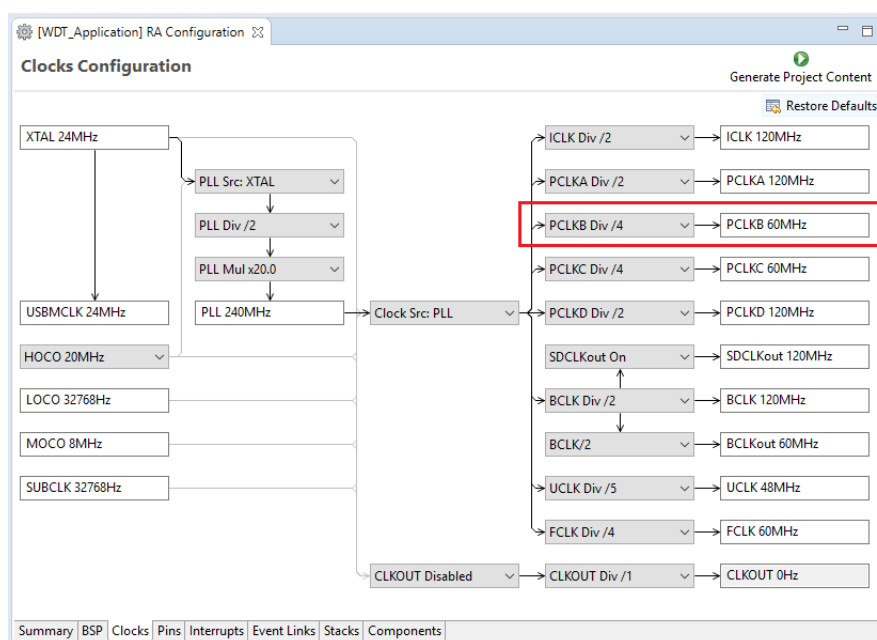
Figure 87: Clock configuration
