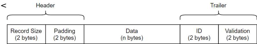
Figure 159: Record Format
