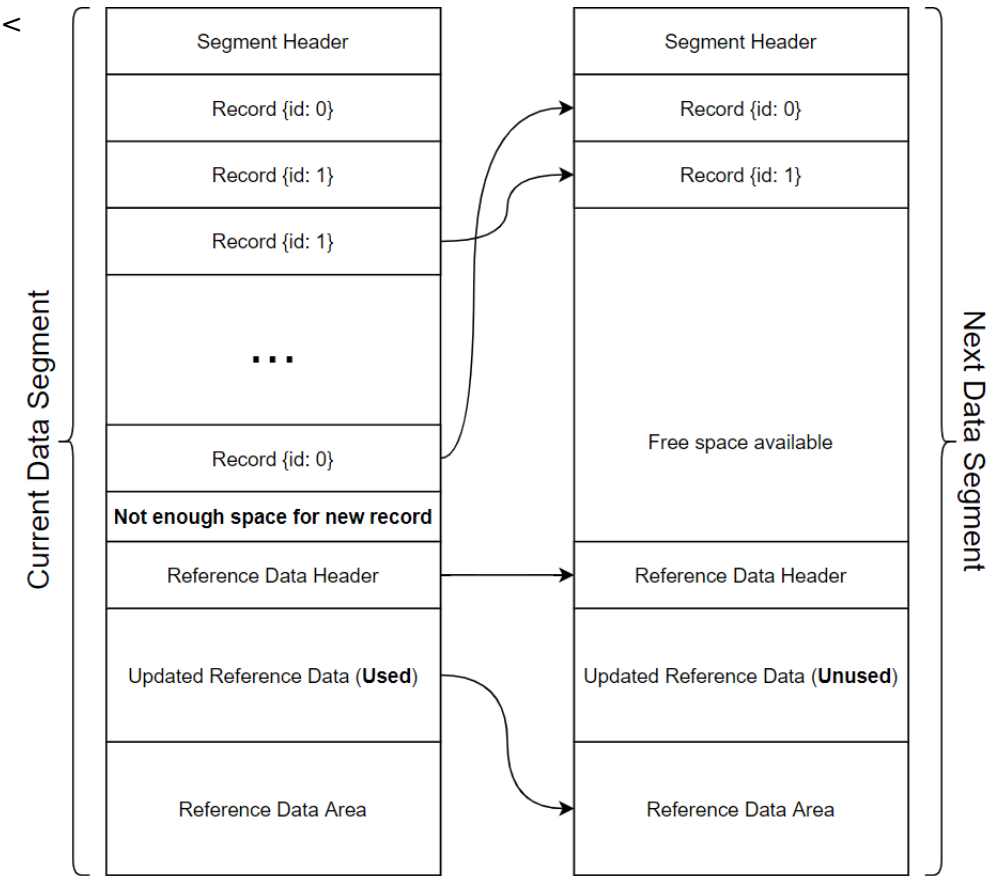
Figure 158: Refresh Operation
