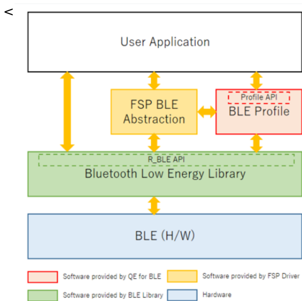
Figure 121: BLE software structure
