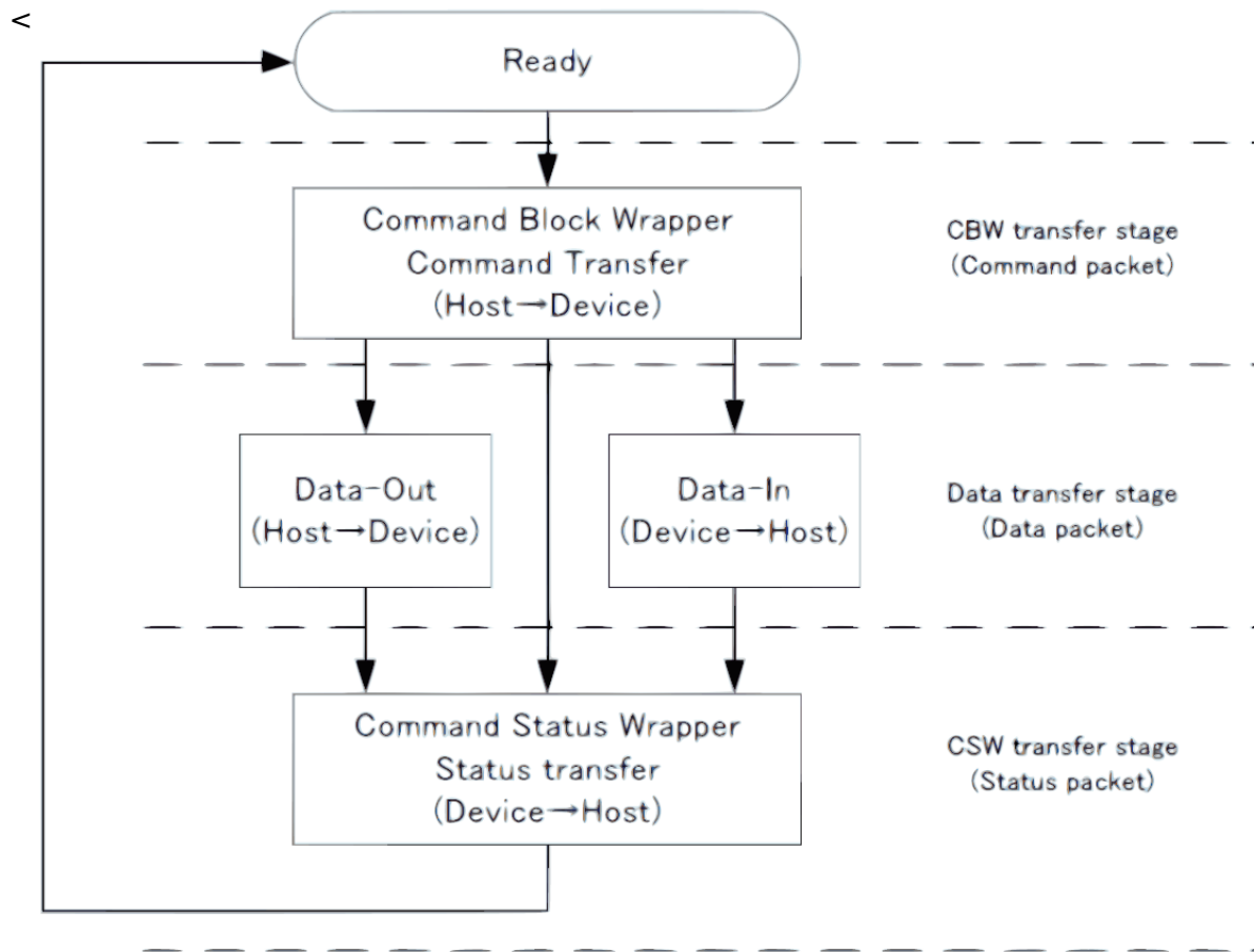
Figure 152: BOT protocol Overview
