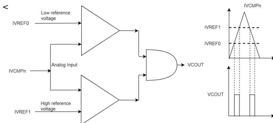
Figure 117: ACMPLP Window Mode Operation
