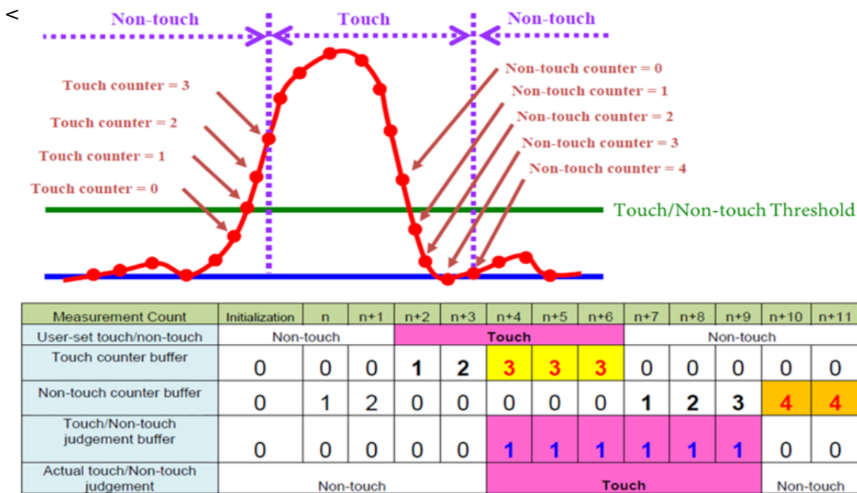
Figure 156: Touch/Non-touch judgement Image
