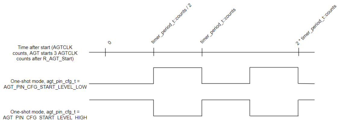
Figure 119: AGT Periodic Output
