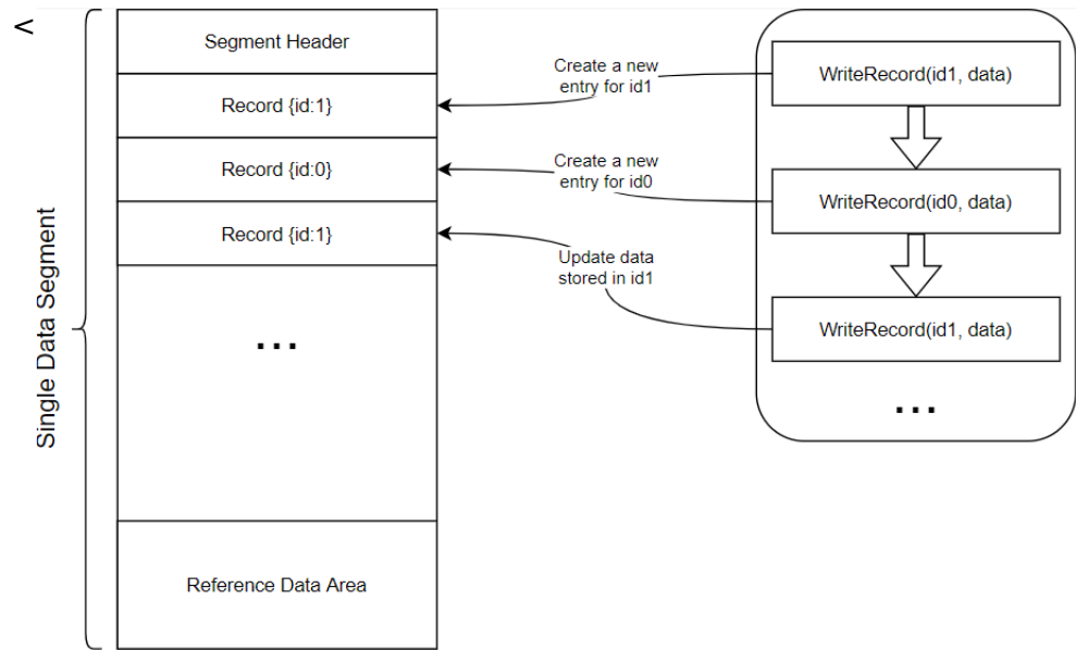
Figure 157: Segment Data Format
