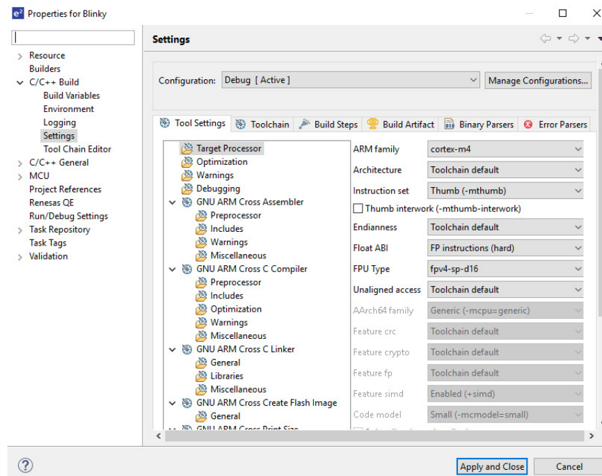
Figure 52: e2 studio Project toolchain settings
