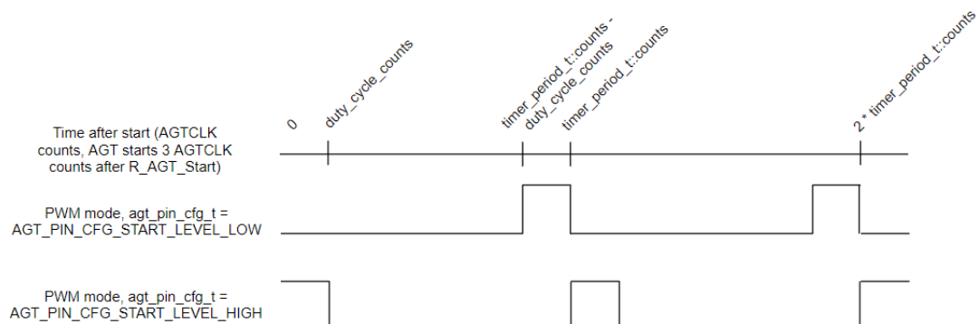
Figure 120: AGT PWM Output
