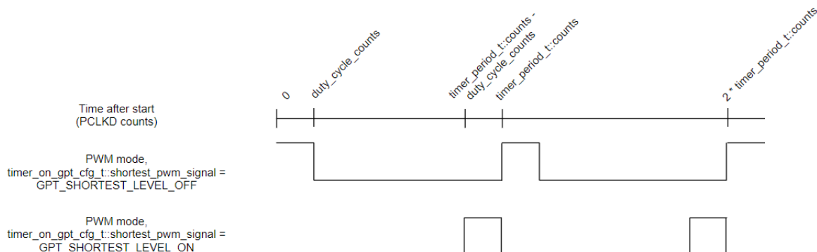
Figure 135: GPT PWM Output
