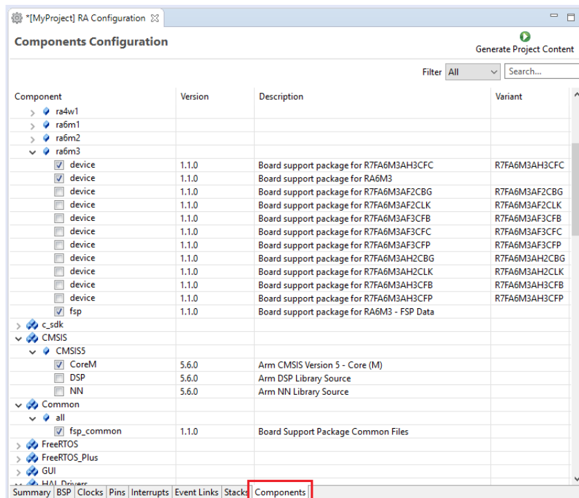
Figure 33: Components Tab
