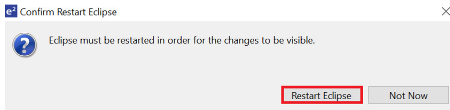
Figure 57: Restart Eclipse
