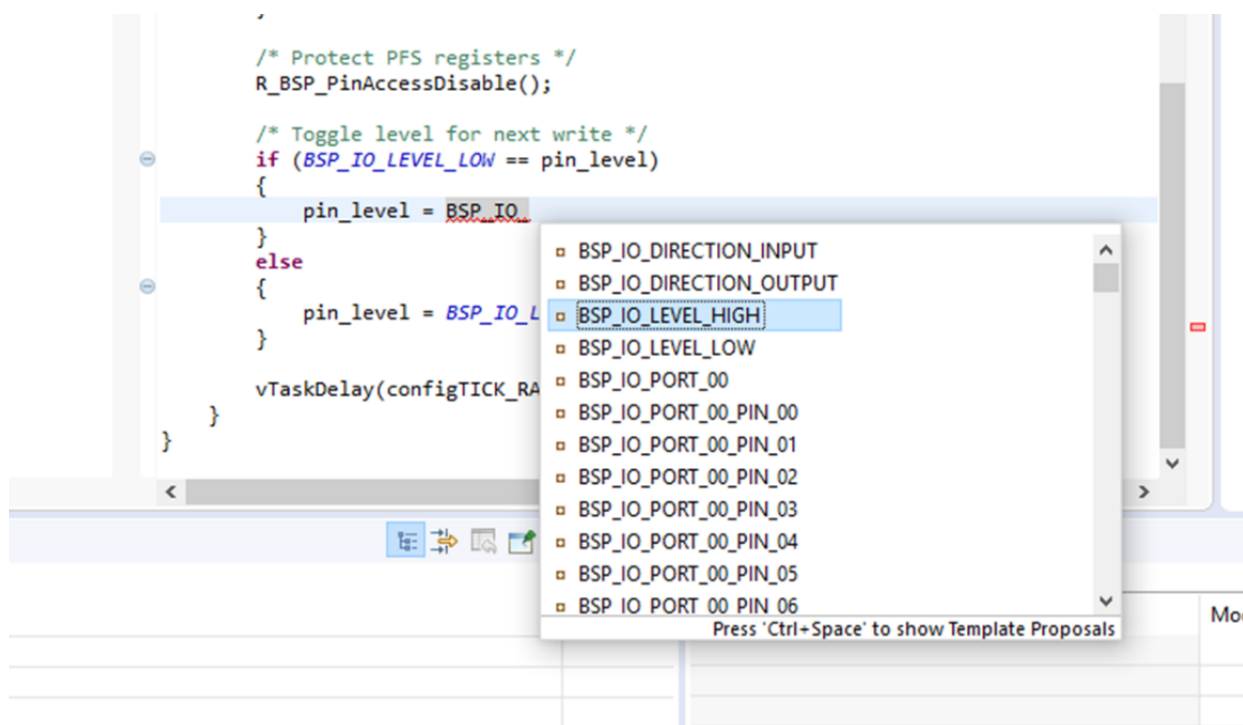
Figure 34: Autocomplete example
