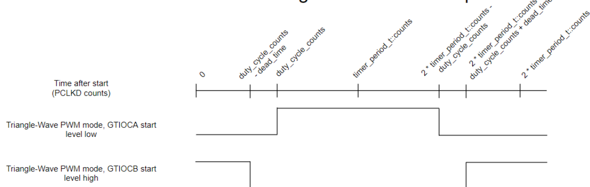
Figure 136: GPT Triangle-Wave PWM Output
