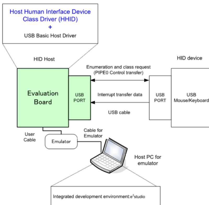
Figure 130: Example Operating Environment
