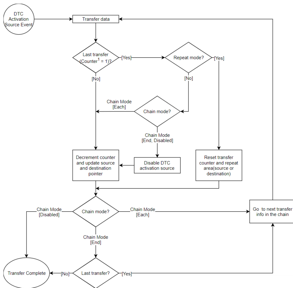
Figure 114: DTC Transfer Flowchart
