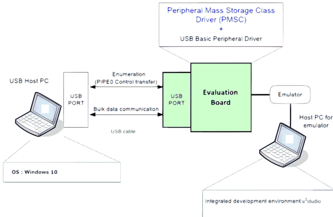
Figure 141: Example Operating Environment
