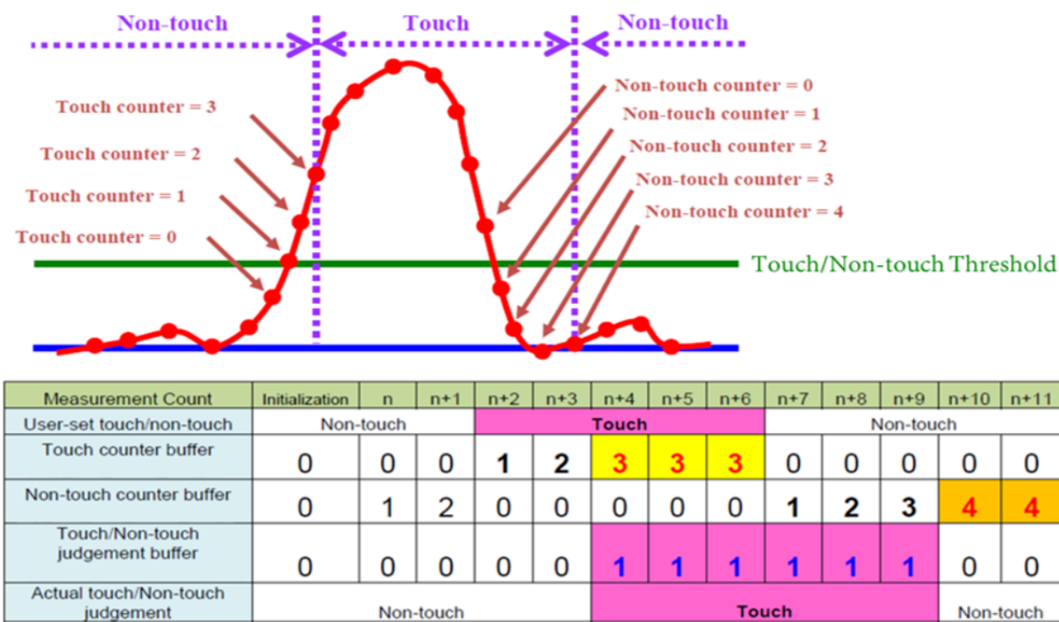
Figure 143: Touch/Non-touch judgement Image
