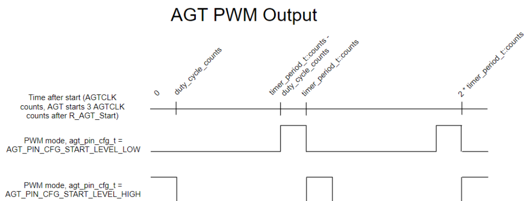
Figure 108: AGT PWM Output
