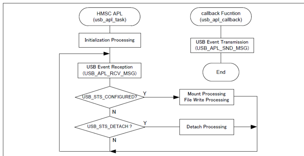
Figure 134: usb_apl_task
