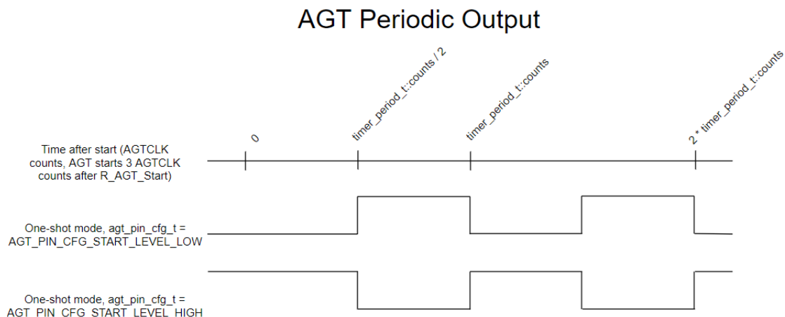
Figure 107: AGT Periodic Output
