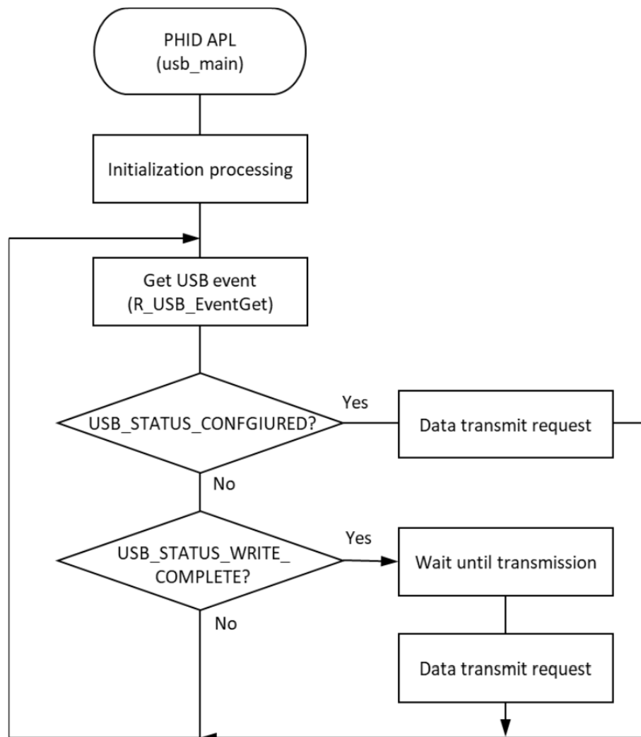
Figure 138: Main Loop processing for OS less
