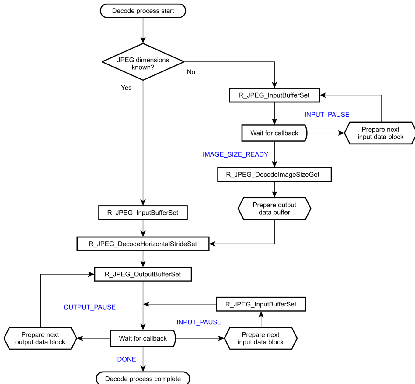
Figure 123: JPEG Decode Operational Flow
