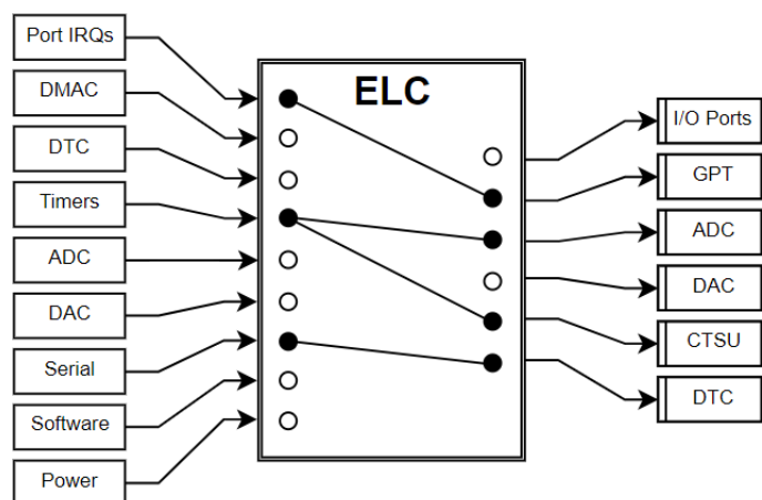
Figure 112: Event Link Controller Conceptual Diagram
