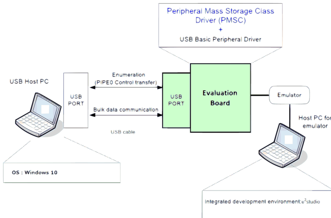
Figure 132: Example Operating Environment
