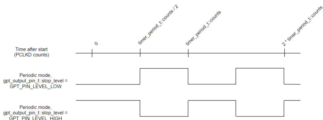
Figure 119: GPT Periodic Output
