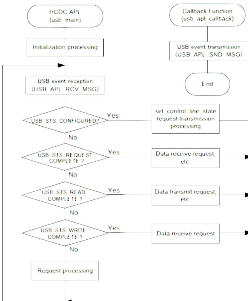
Figure 126: Main Loop processing (for RTOS)
