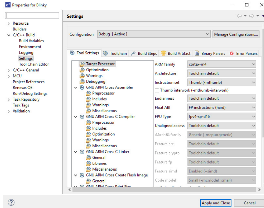
Figure 46: e2 studio Project toolchain settings
