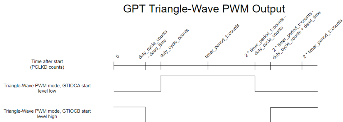
Figure 121: GPT Triangle-Wave PWM Output
