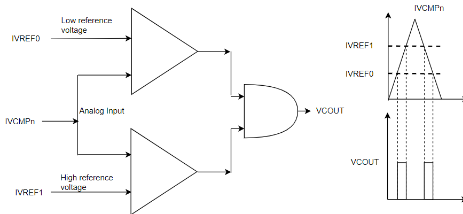
Figure 105: ACMPLP Window Mode Operation
