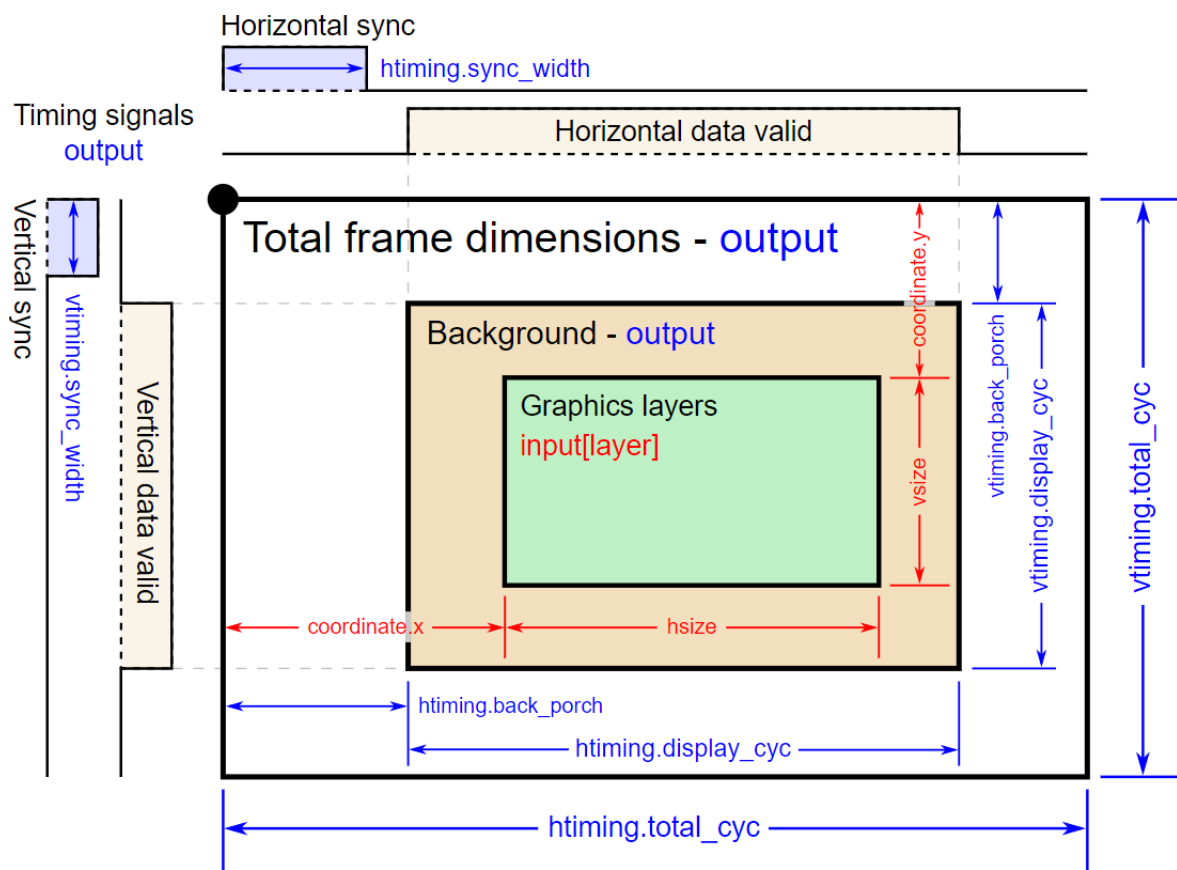
Figure 117: GLCDC layers and timing
