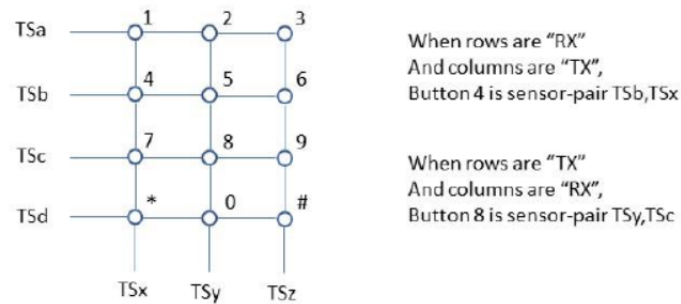
Figure 109: Mutual Button Image
