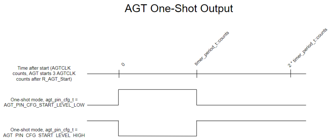
Figure 106: AGT One-Shot Output
