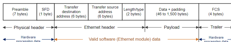
Figure 114: Frame Format Image
