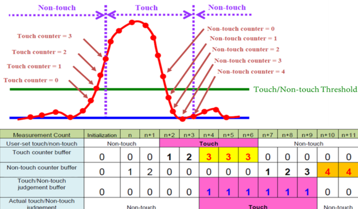
Figure 134: Touch/Non-touch judgement Image
