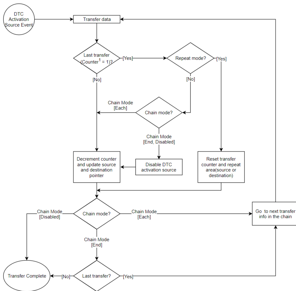
Figure 111: DTC Transfer Flowchart
