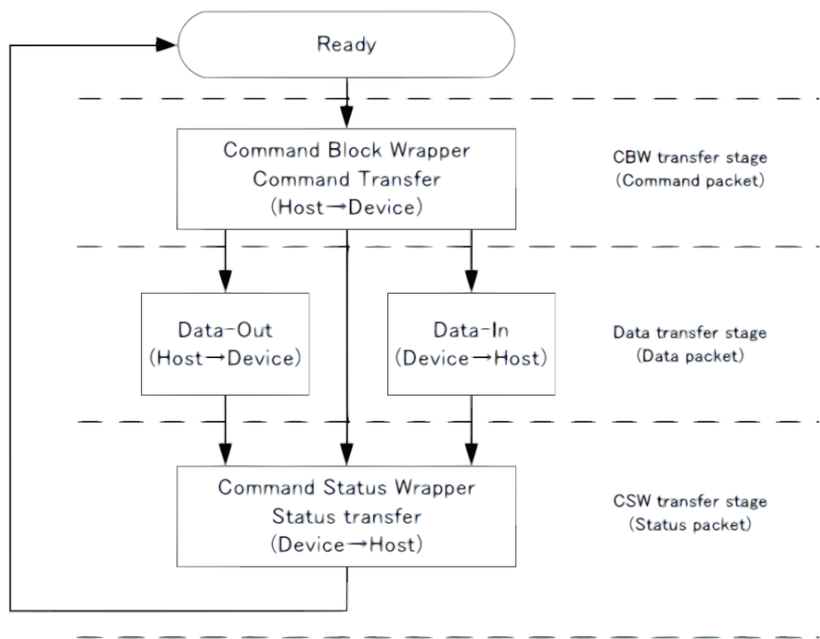
Figure 131: BOT protocol Overview
