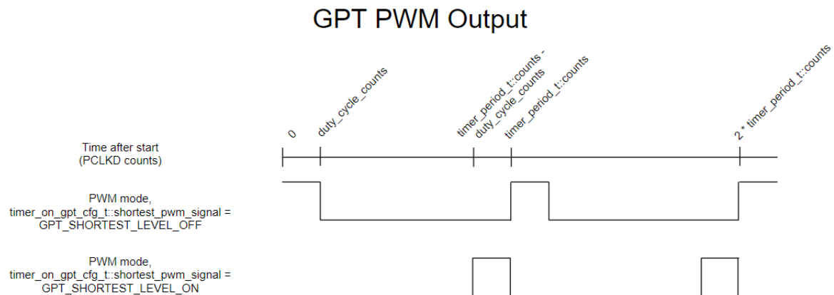
Figure 120: GPT PWM Output
