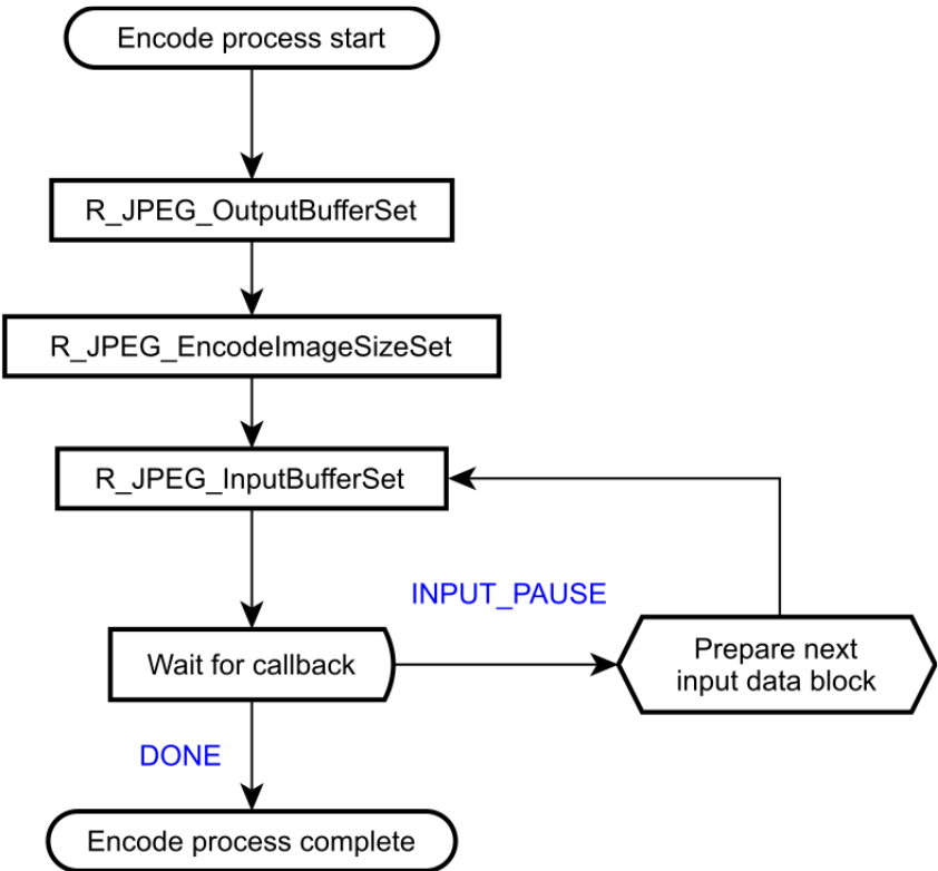
Figure 124: JPEG Encode Operational Flow
