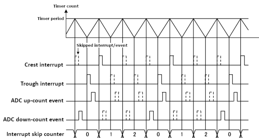
Figure 122: Crest interrupt skipping in triangle-wave PWM modes (skip count 2)
