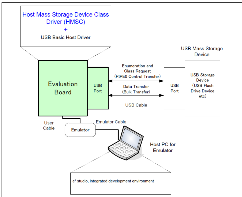
Figure 127: Example Operating Environment
