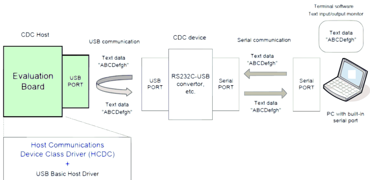
Figure 125: Data Transfer (Loopback)
