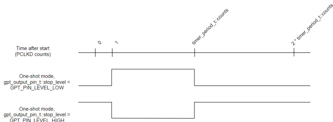
Figure 118: GPT One-Shot Output
