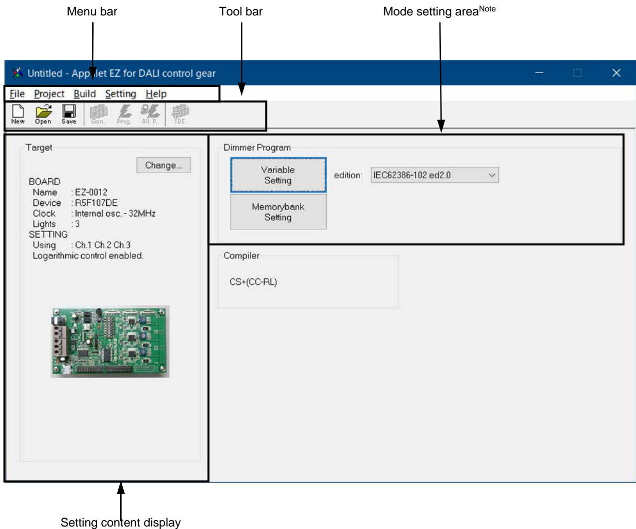
Figure5-1 Main Window
