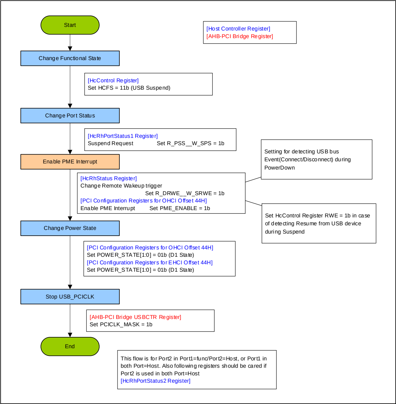
Figure 10.13 Host Controller Power-Down Flow (When Using OHCI)
