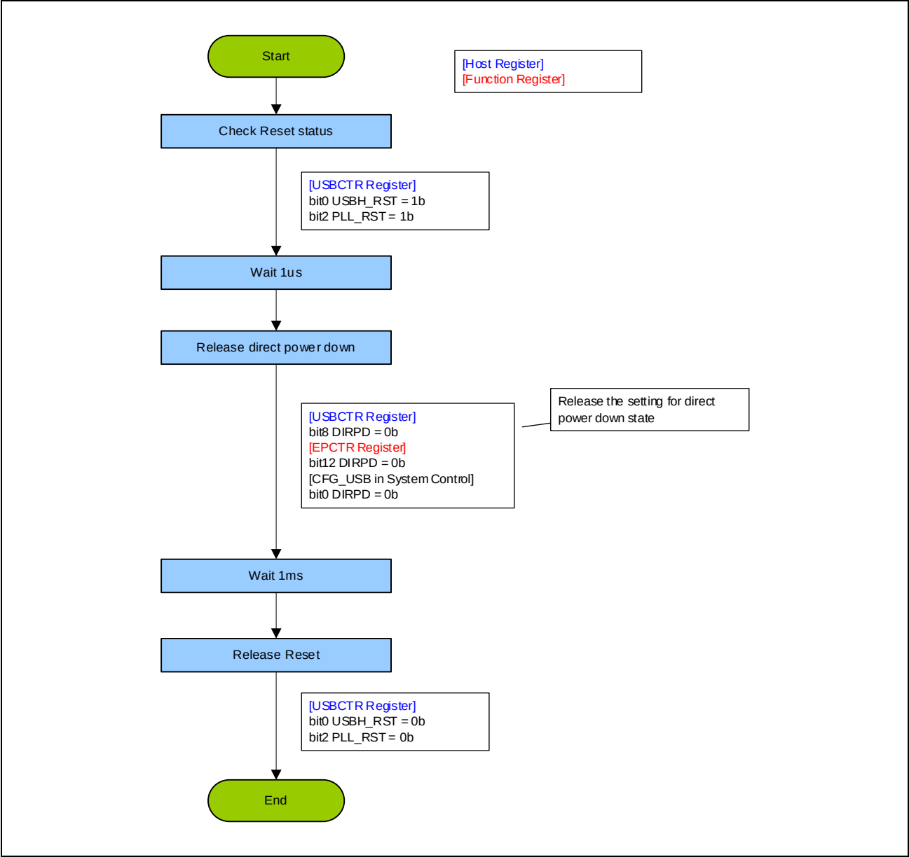
Figure 10.22 Exiting the Direct Power-Down Mode (Host Controller)
