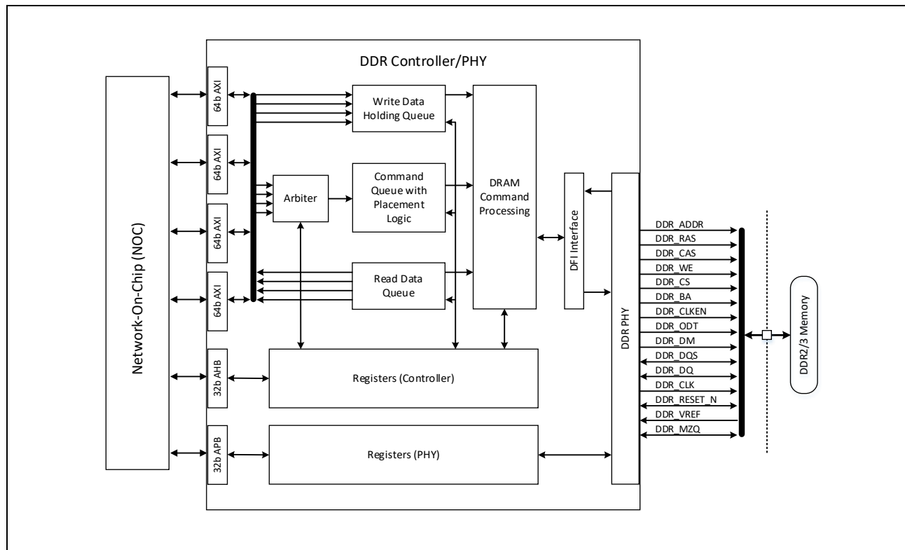
Figure 6.1 DDR Controller Interfaces and Connections
