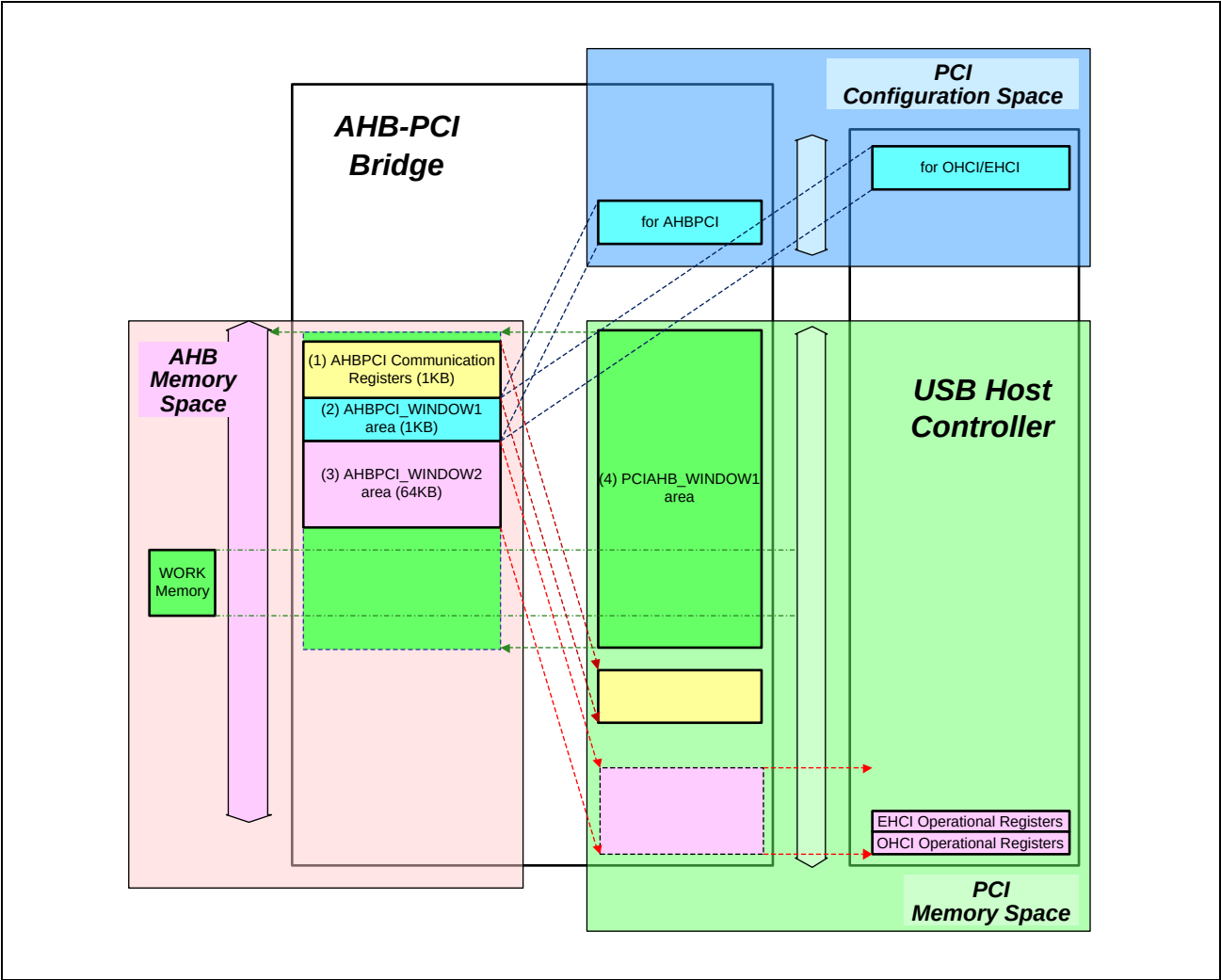
Figure 10.4 AHB and PCI Space Mapping Image (Areas Overlapping)
