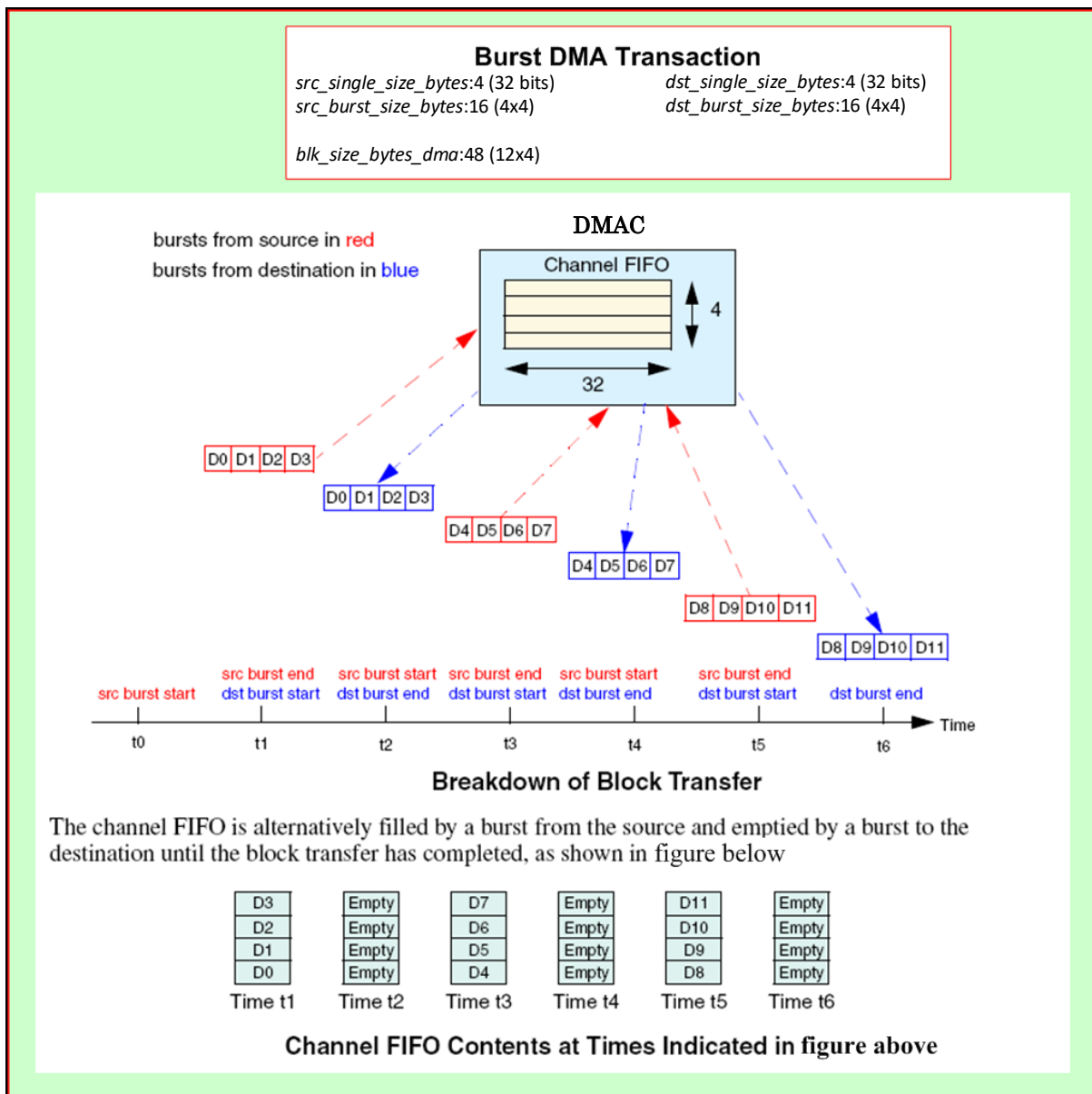
Figure 11.4 Burst DMA Transaction
