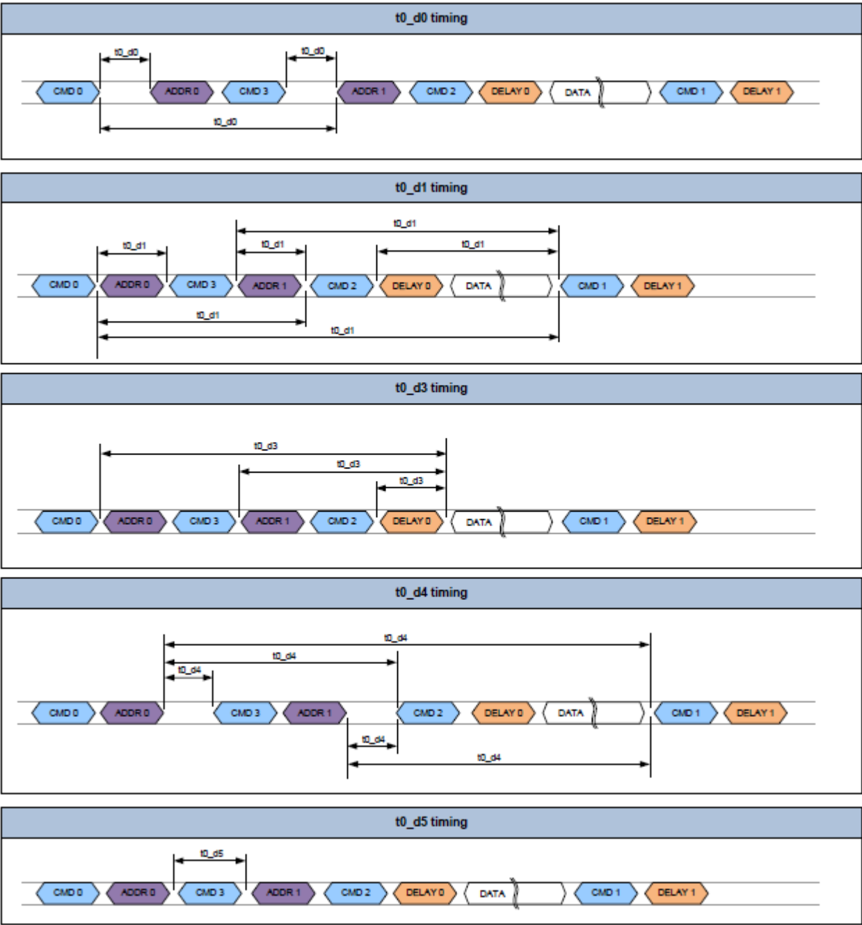
Figure 7.26 Generic Sequence Timing Parameters 1
