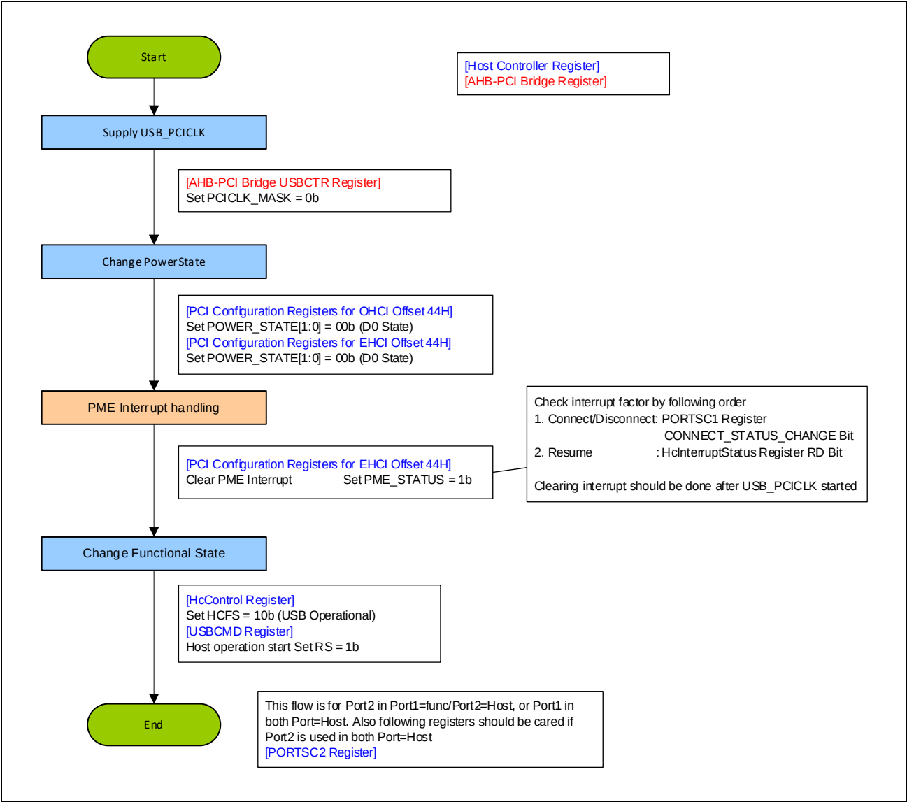
Figure 10.16 Host Controller Power-Up Flow (When Using EHCI)
