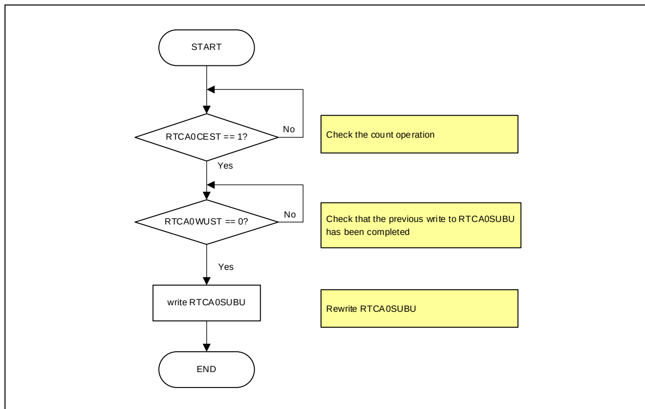
Figure 12.8 Writing to RTCA0SUBU
