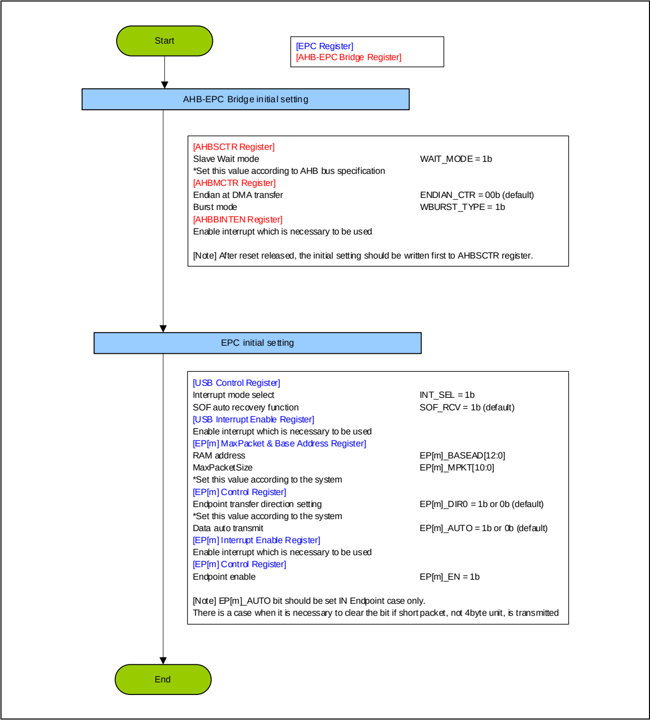
Figure 10.26 Function Controller Initial Setup Sequence
