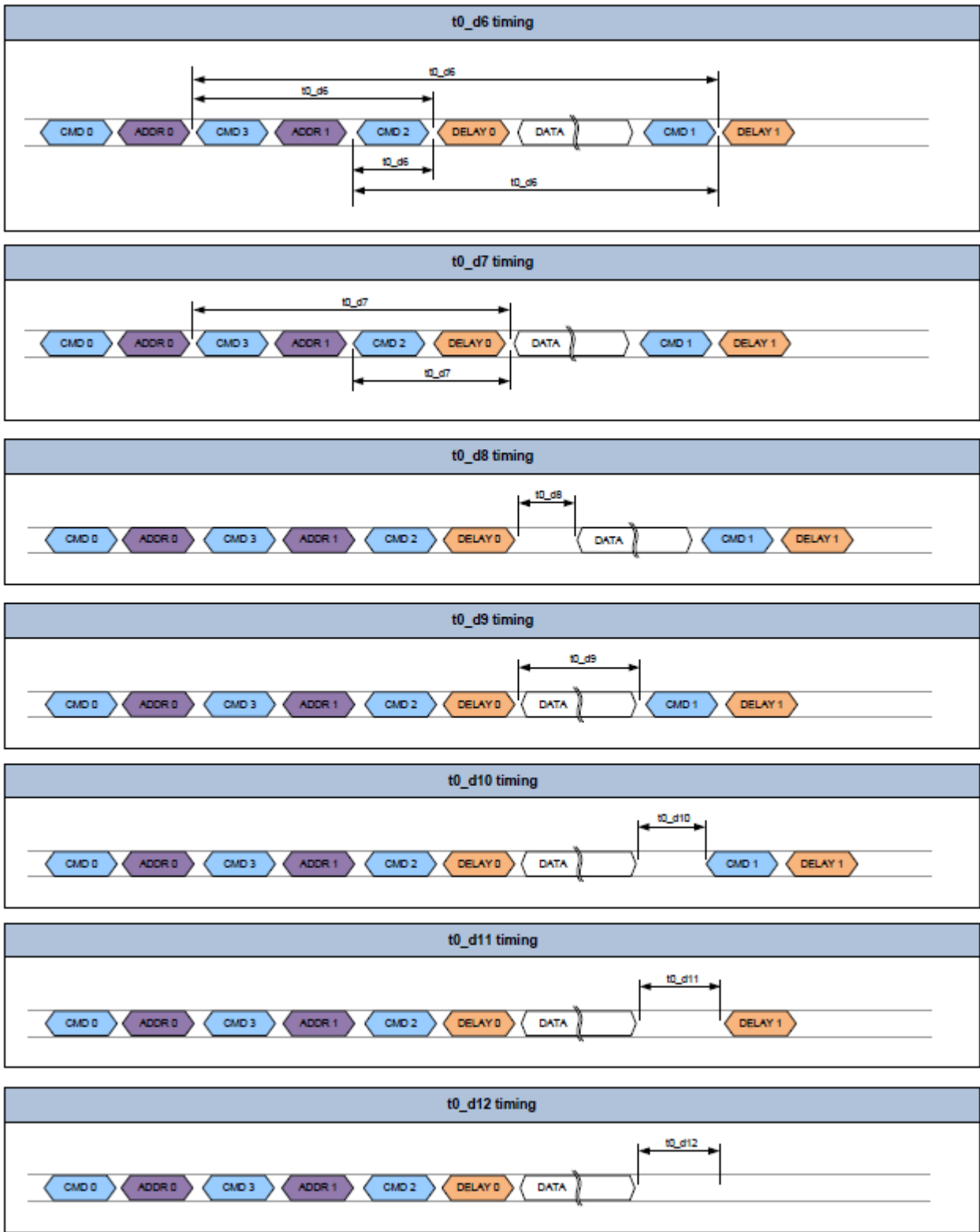
Figure 7.27 Generic Sequence Timing Parameters 2
