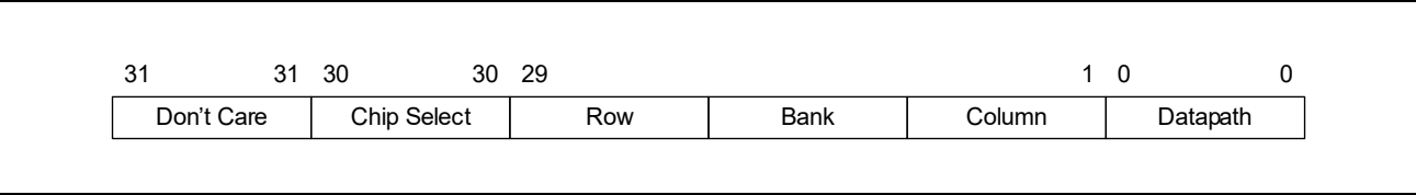
Figure 6.3 Maximum Memory Map
