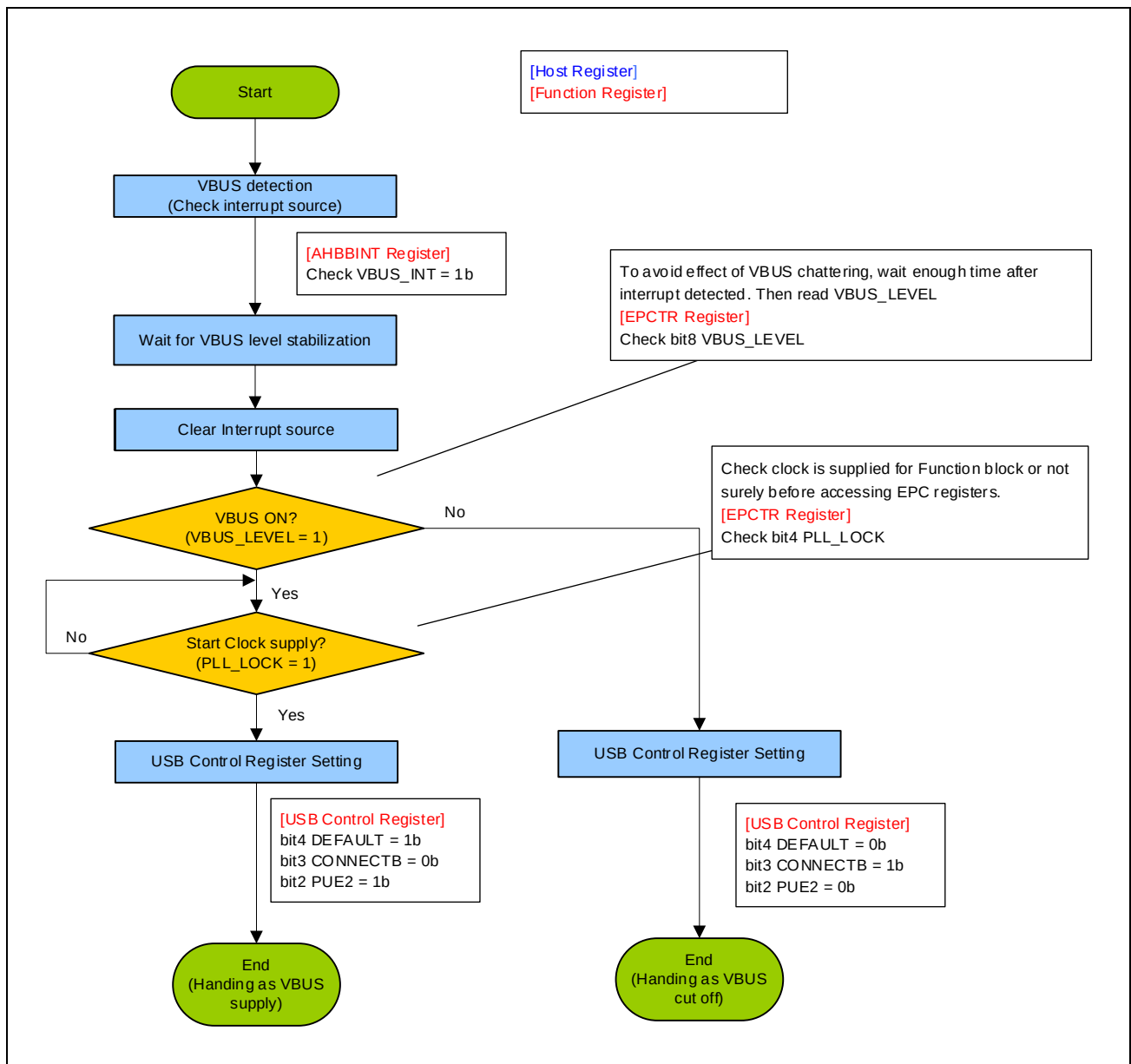
Figure 10.12 VBUS Detection Flow
