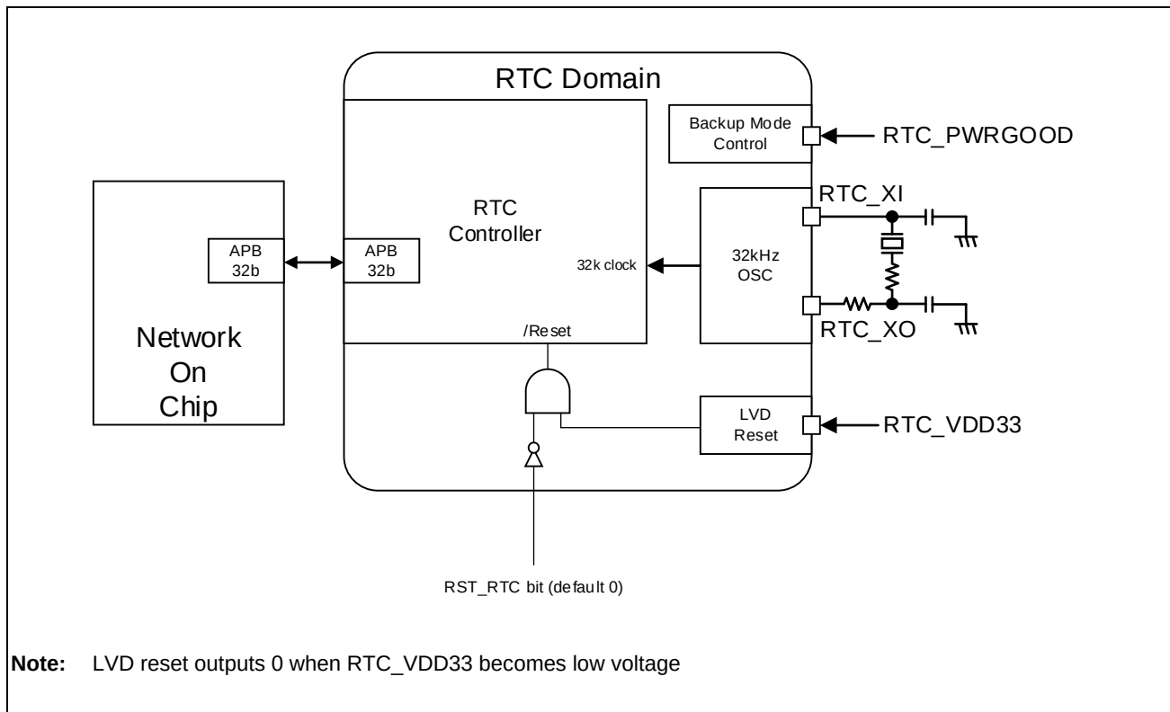
Figure 12.1 RTC Interfaces and Connections
