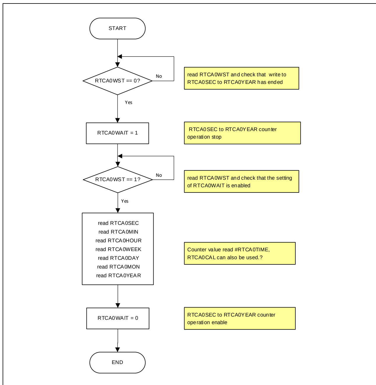
Figure 12.4 Reading RTC Using the Buffer Registers
