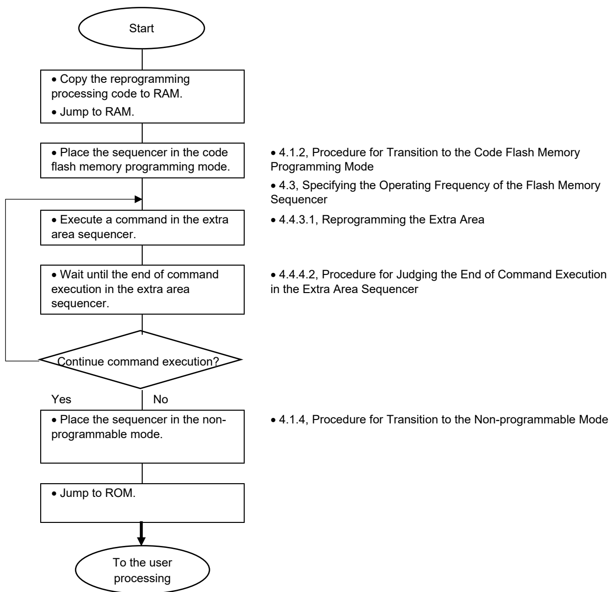
Figure 4-5 Flowchart of Command Execution for Reprogramming of the Extra Area
