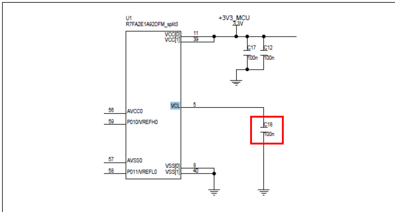
Figure 2. MCU VCL Pin Capacitor Incorrect Value
