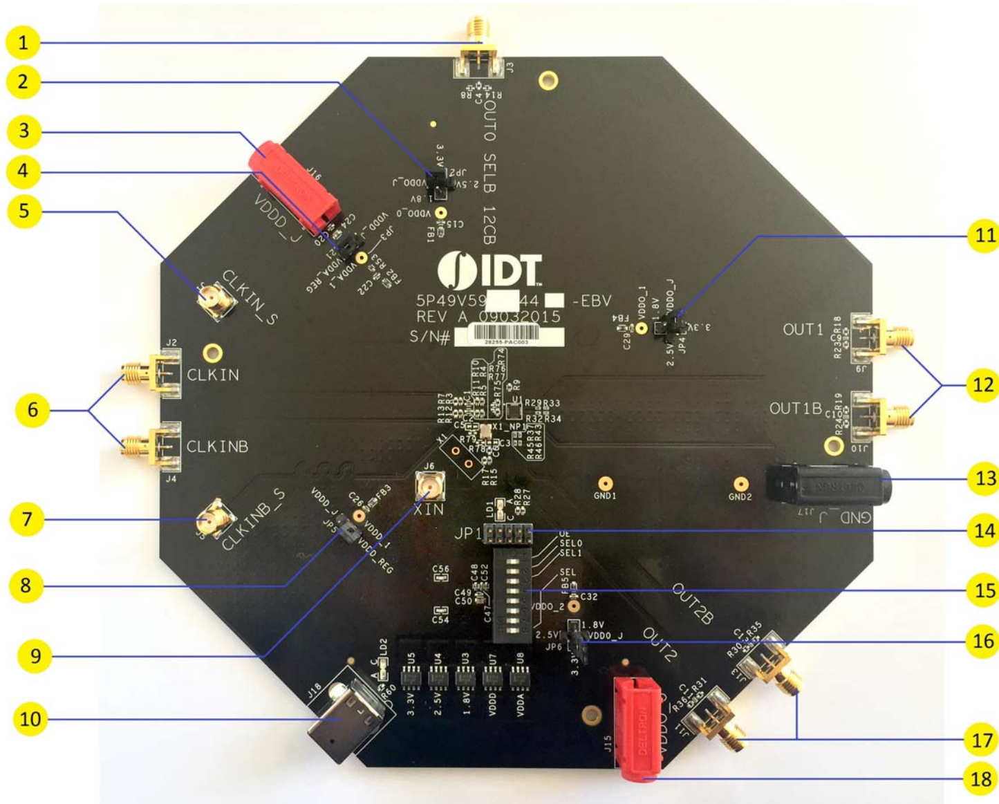
Figure 1. 5P49V5943/44 Evaluation Board
