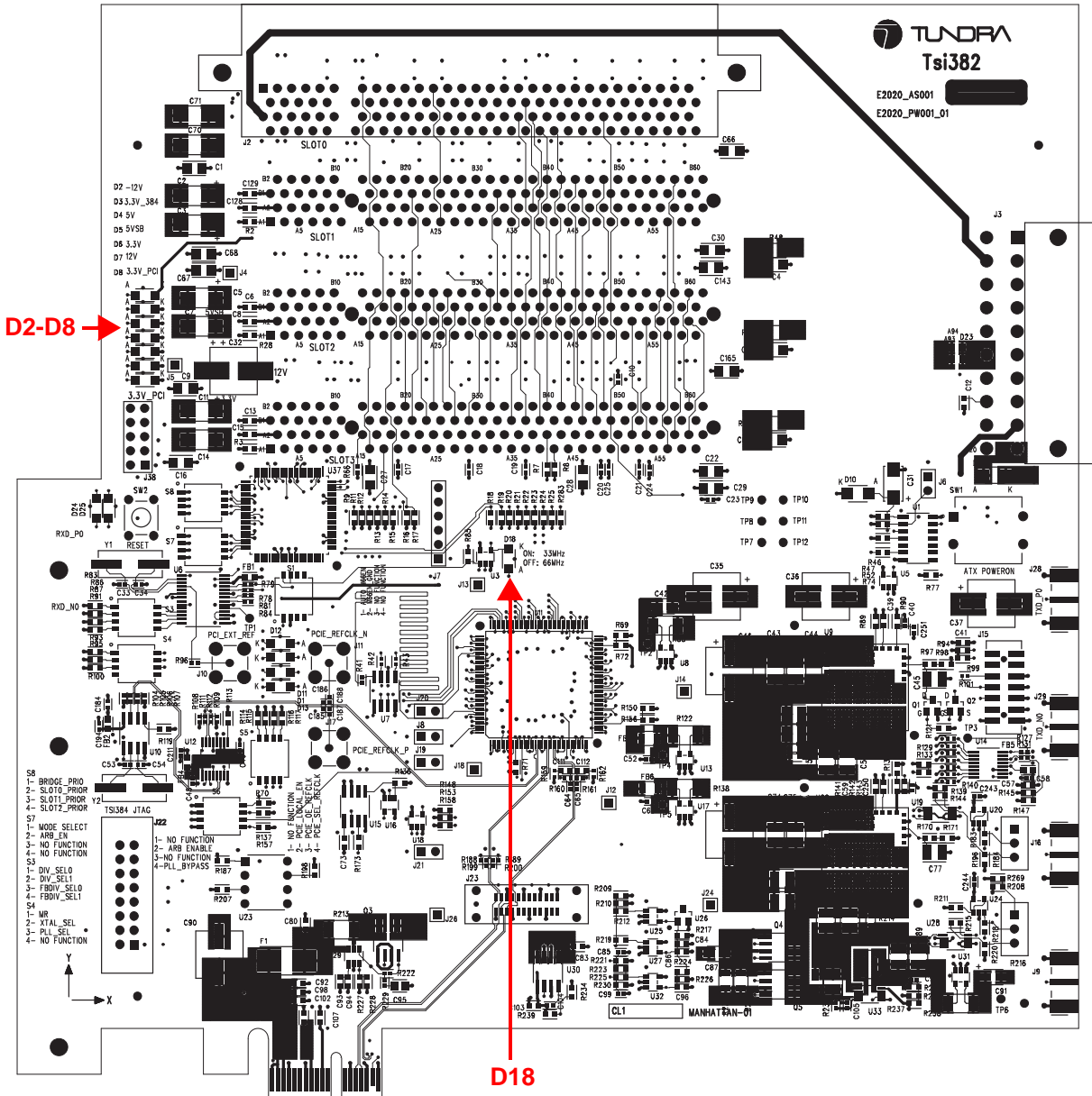
Figure 10: LED Locations
