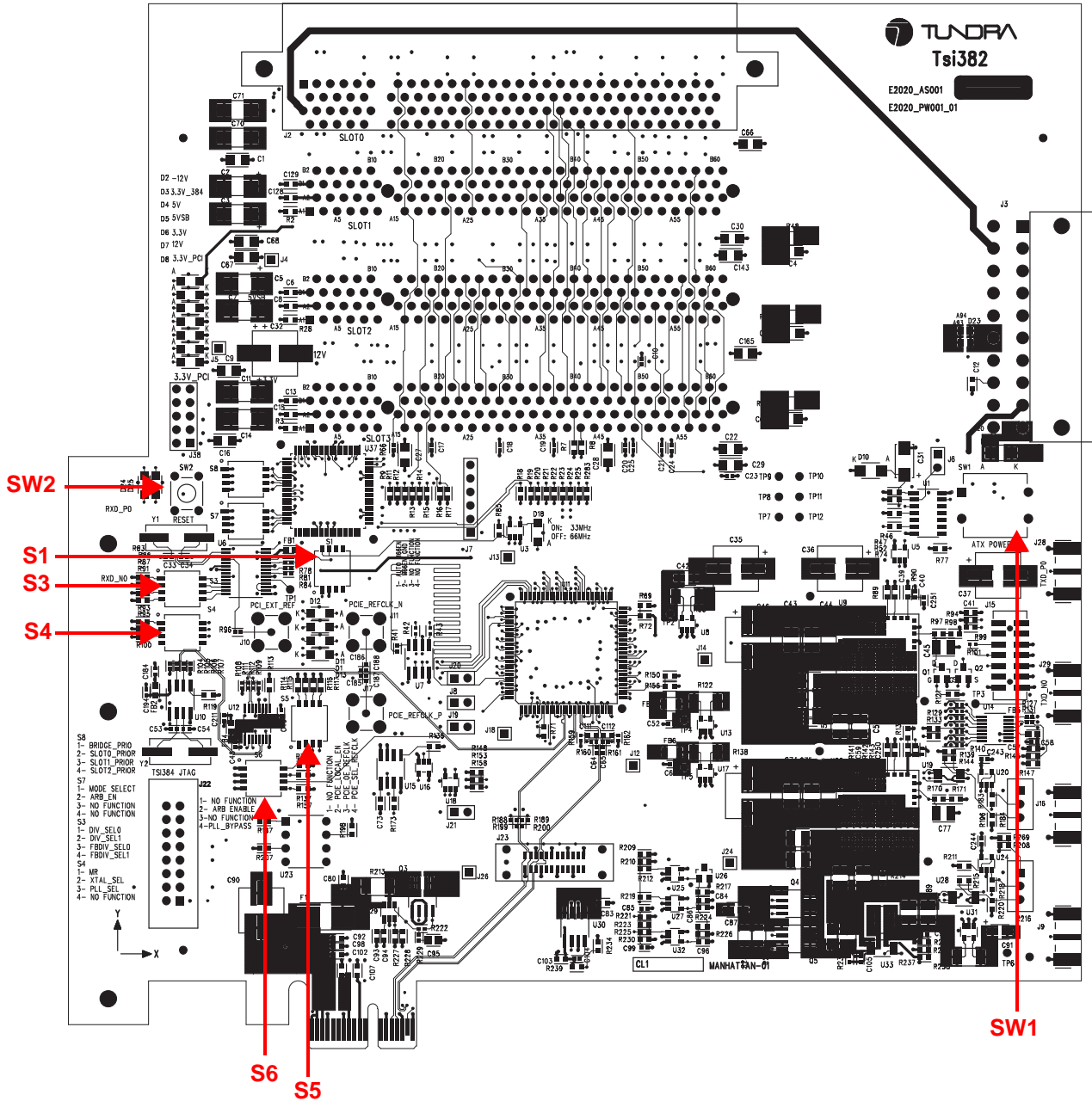
Figure 6: Switch Locations
