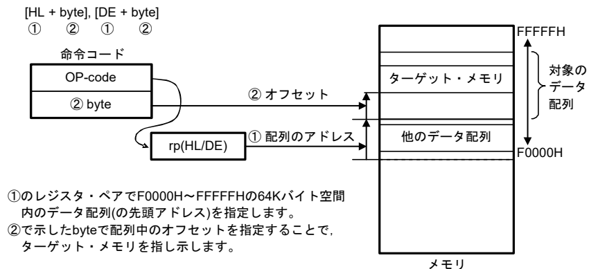
図3 - 28 [HL+byte], [DE+byte]の例
