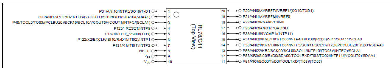
Figure 2.2 RL78/G11 (20-pin Products) Pin Configuration
