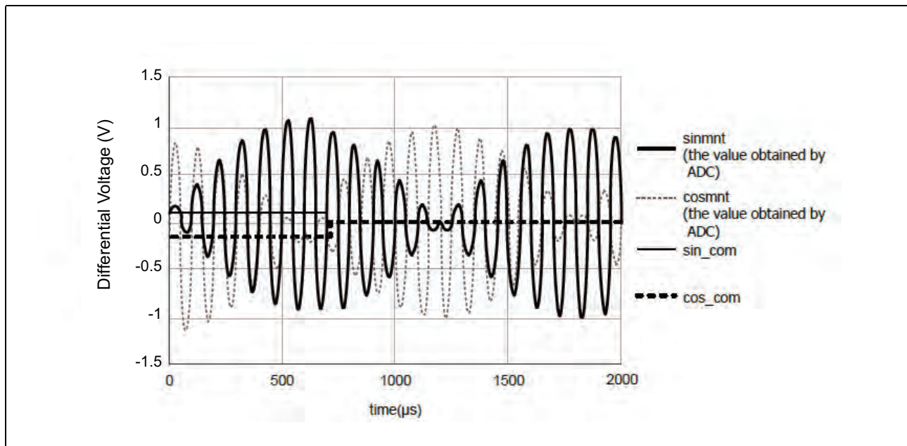
Figure 49.46 Correction of Common Offsets
