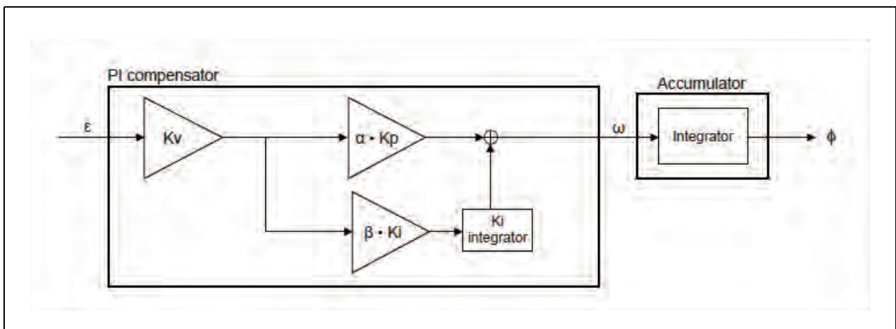
Figure 49.35 PI Compensator and Accumulator
