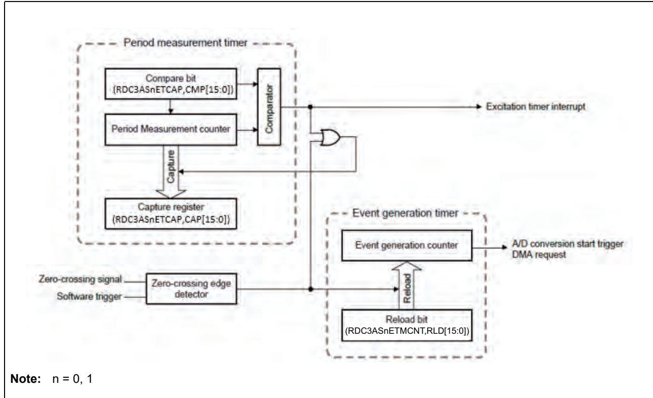
Figure 49.56 Block Diagram of Excitation Timer
