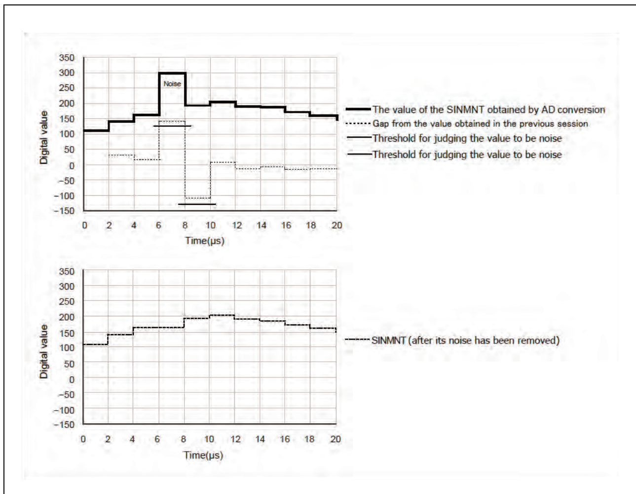
Figure 49.7 Judging and Eliminating Noise
