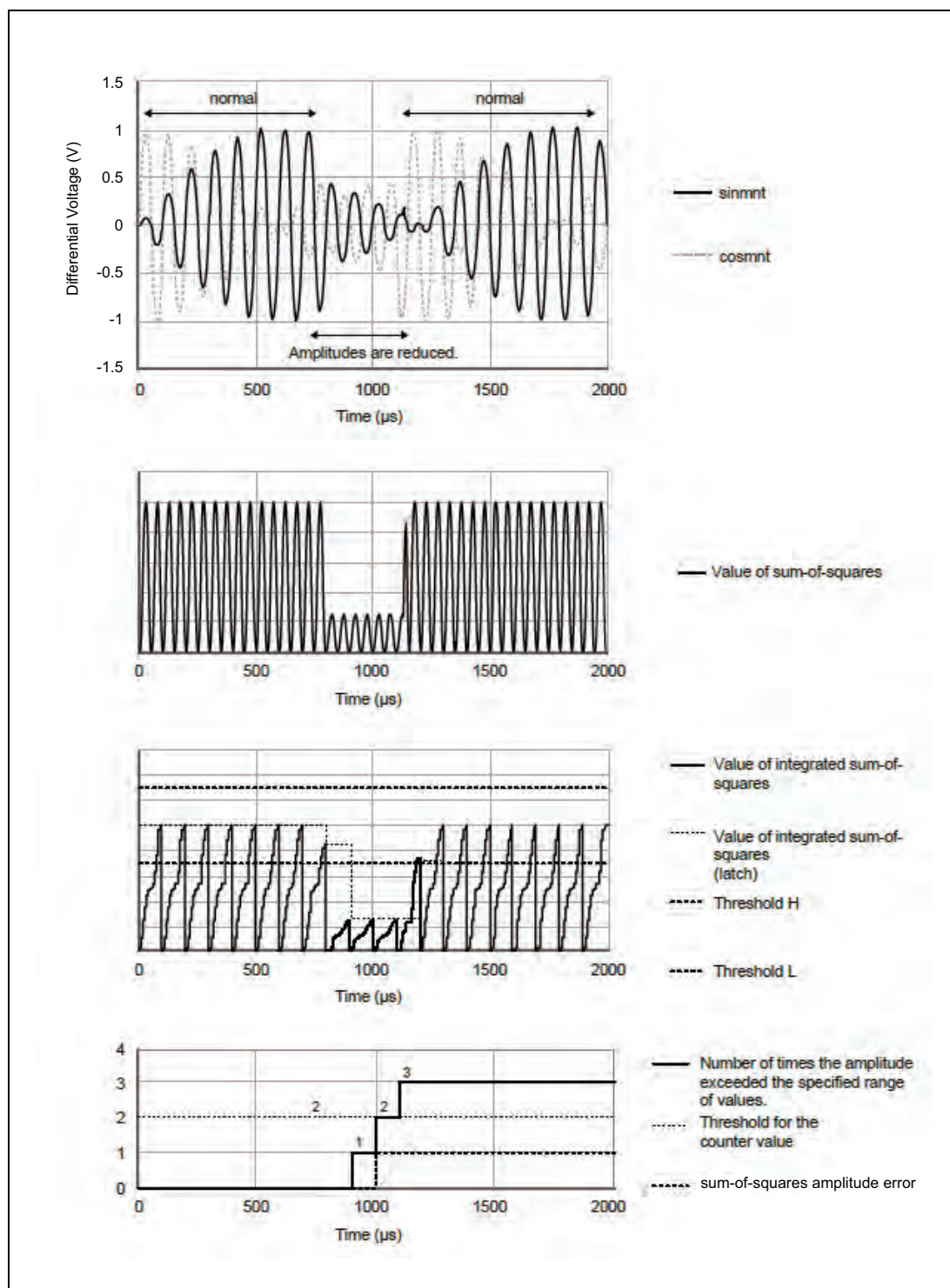
Figure 49.53 Example of Waveforms with Sum-of-Squares Amplitude Error
