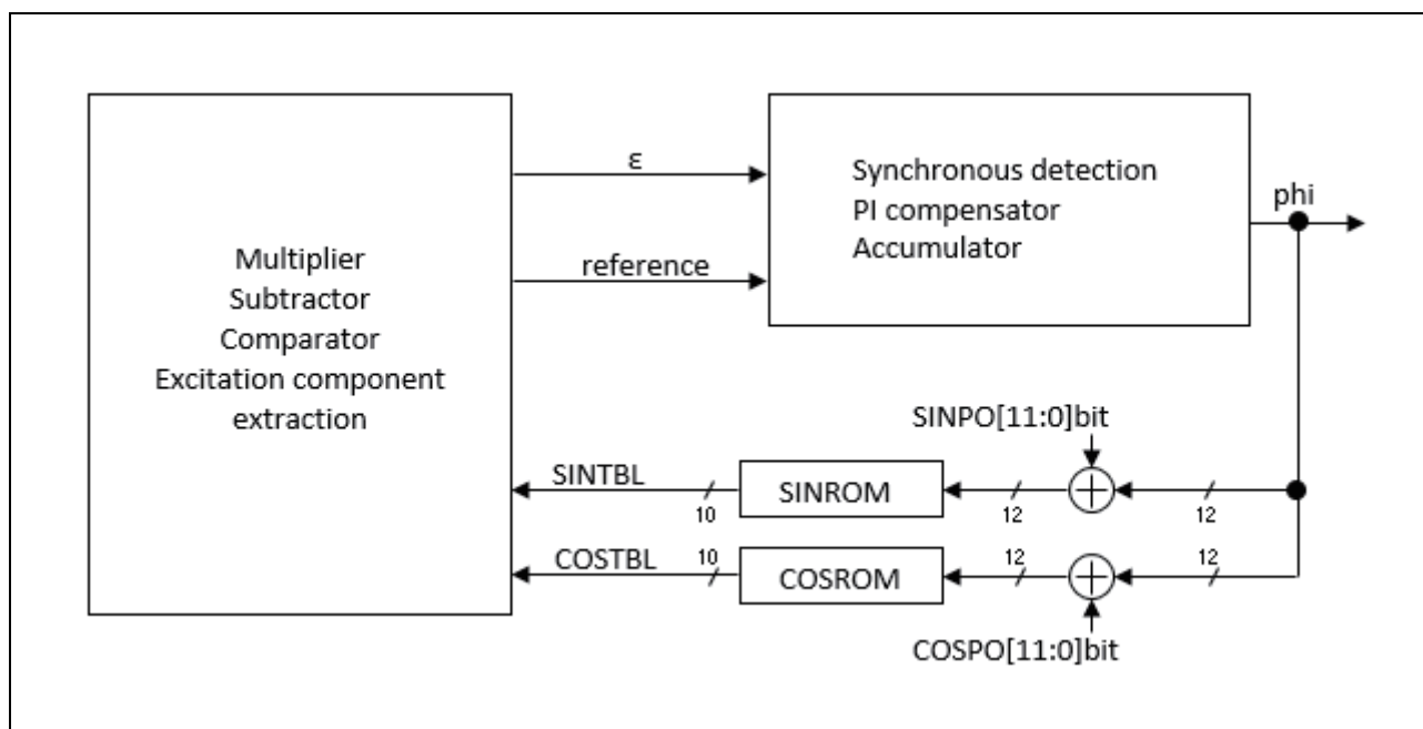
Figure 49.12 Structure of Sine and Cosine Angle Correction Circuit
