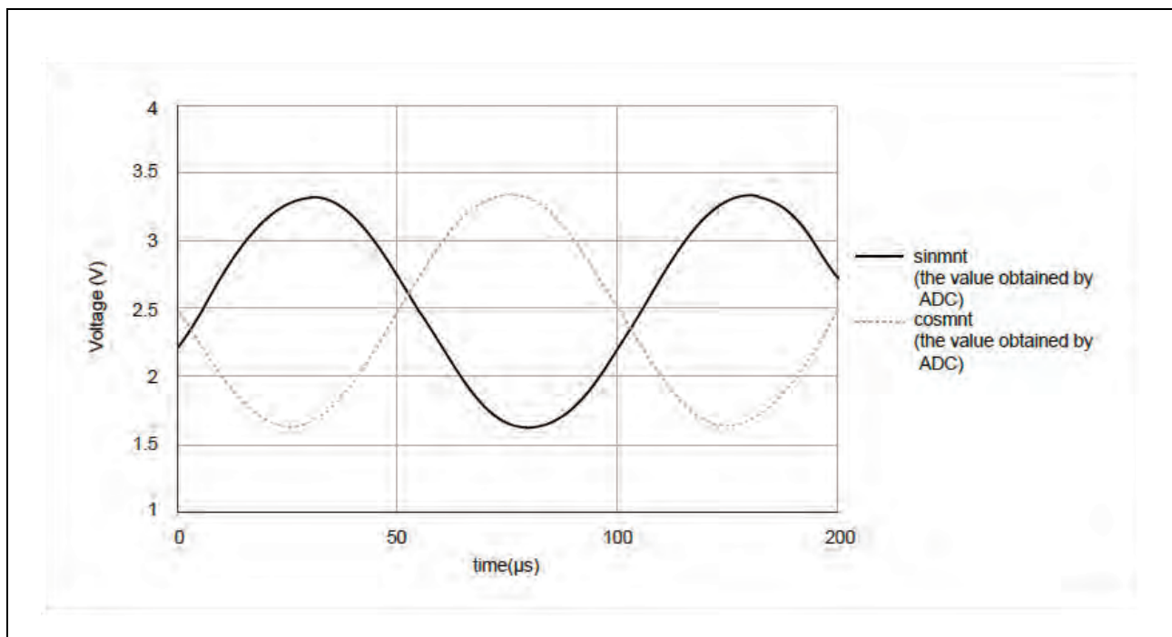
Figure 49.10 Signal with Delay
