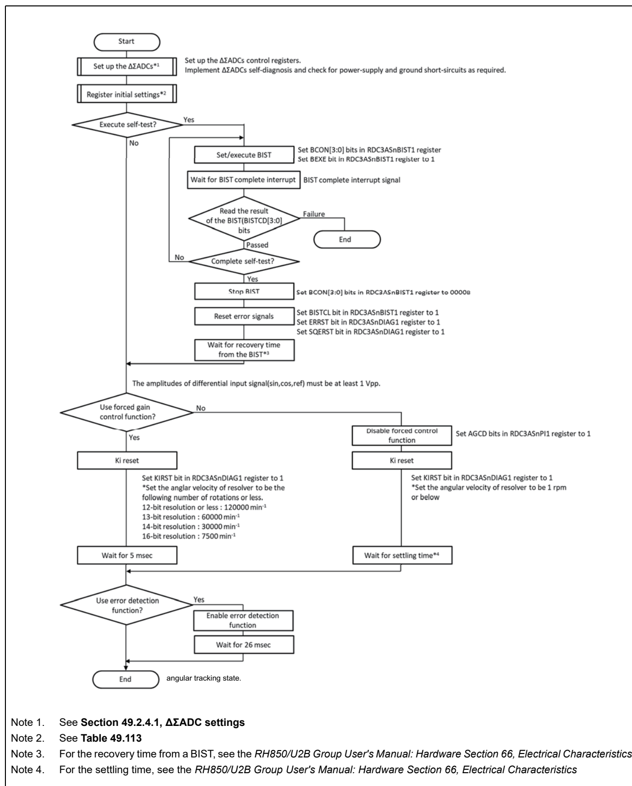
Figure 49.59 RDC3AS Initial Operation Flow
