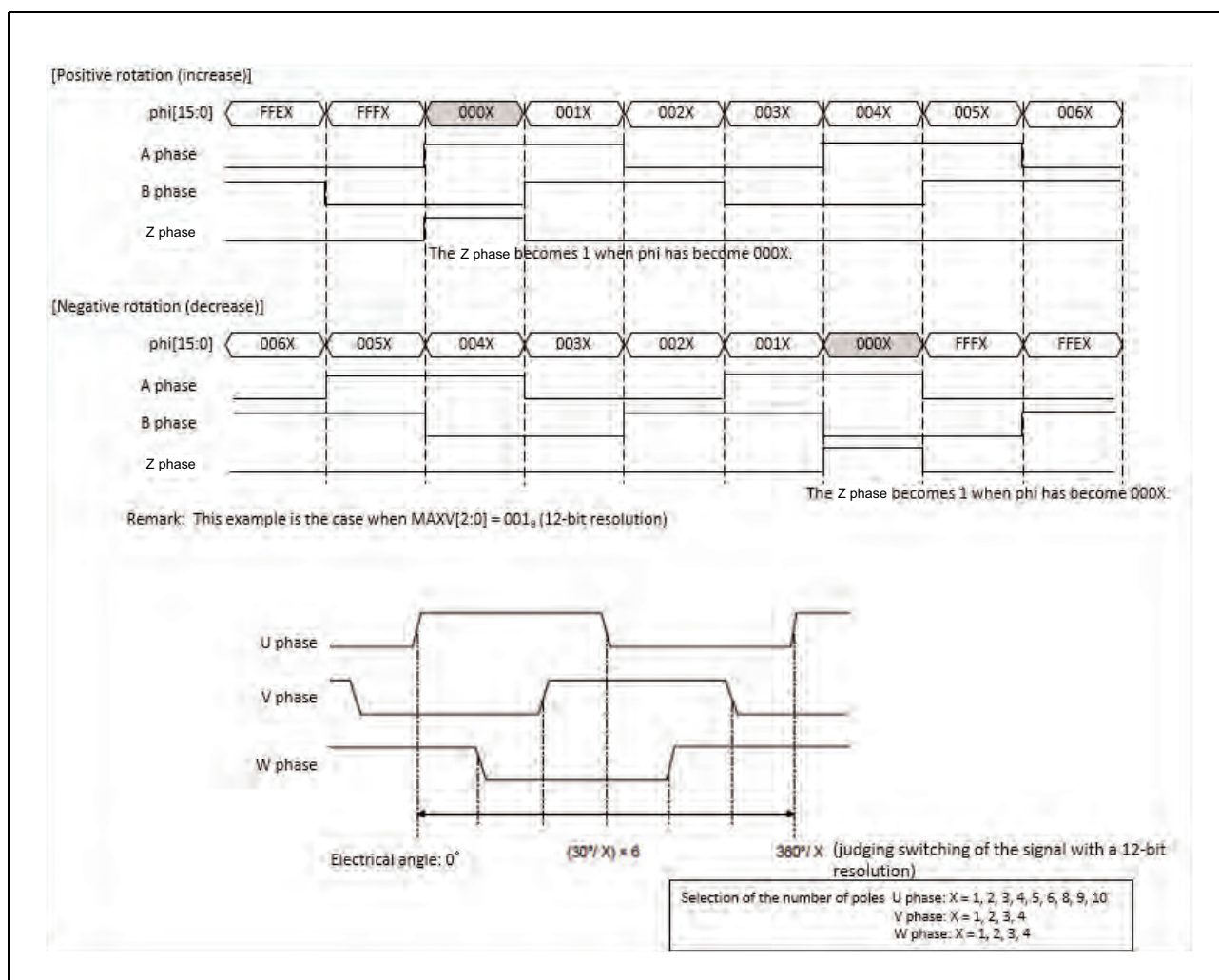
Figure 49.44 Waveforms of Encoder Phase Pulse Operation when Hysteresis is On and Off.
