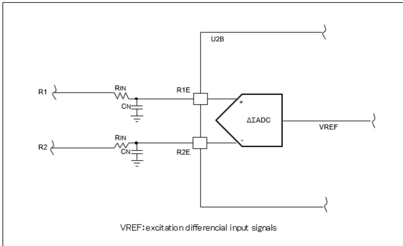
Figure 49.61 Resolver Excitation Signal External Input Circuit
