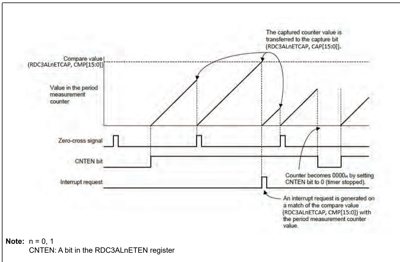
Figure 49.22 Example of Period Measurement Timer Operation
