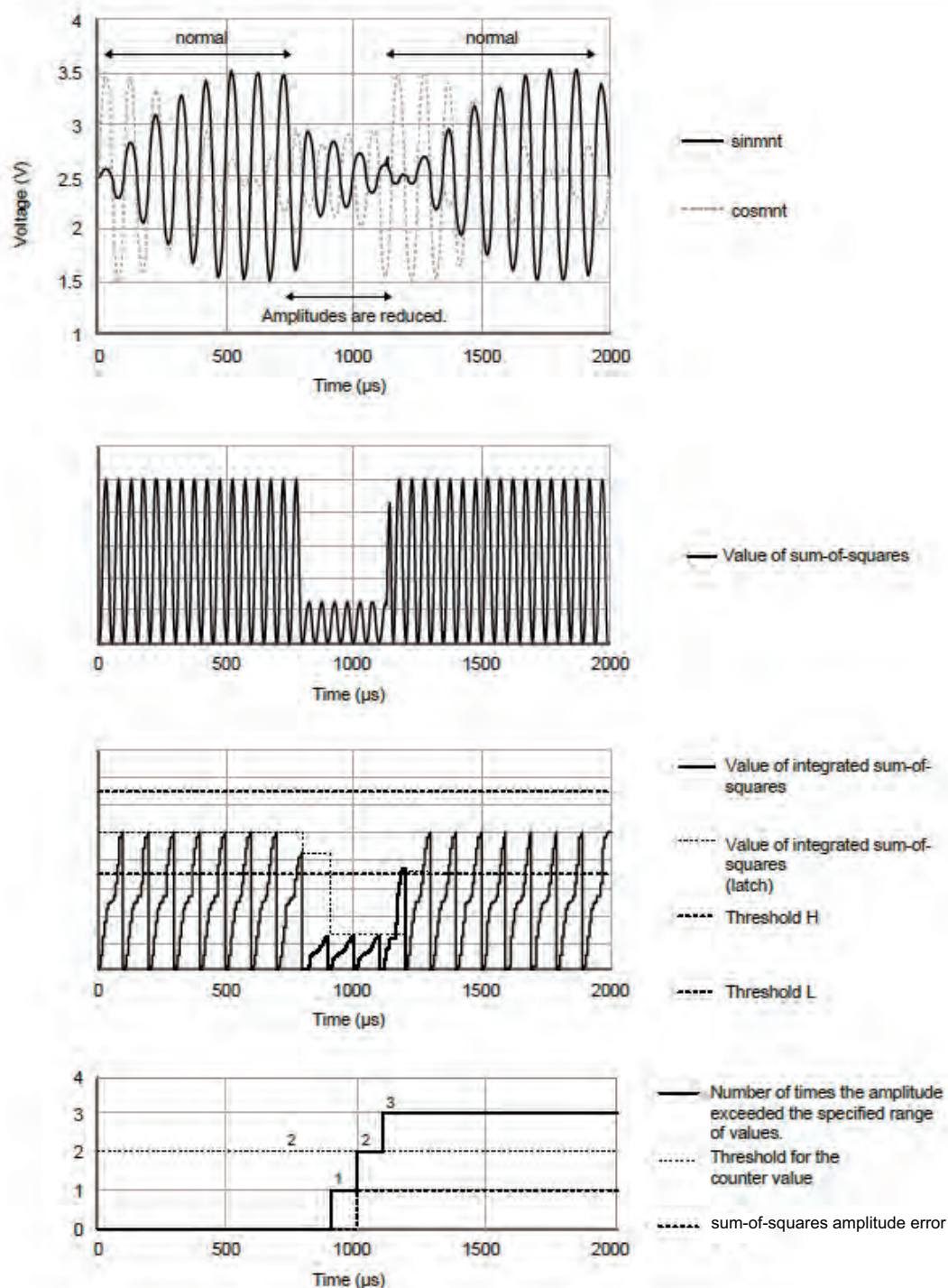
Figure 49.17 Example of Waveforms with Sum-of-Squares amplitude Error
