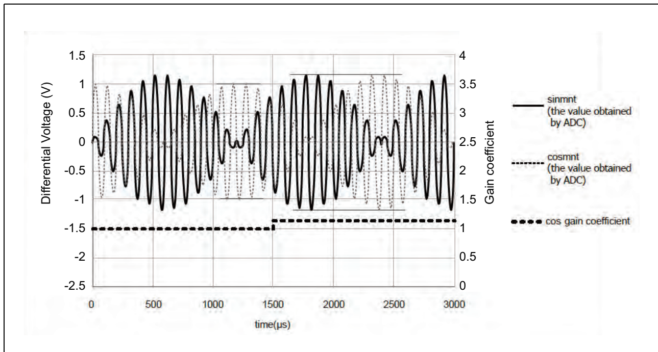
Figure 49.45 Correction to Make the Amplitudes Correspond
