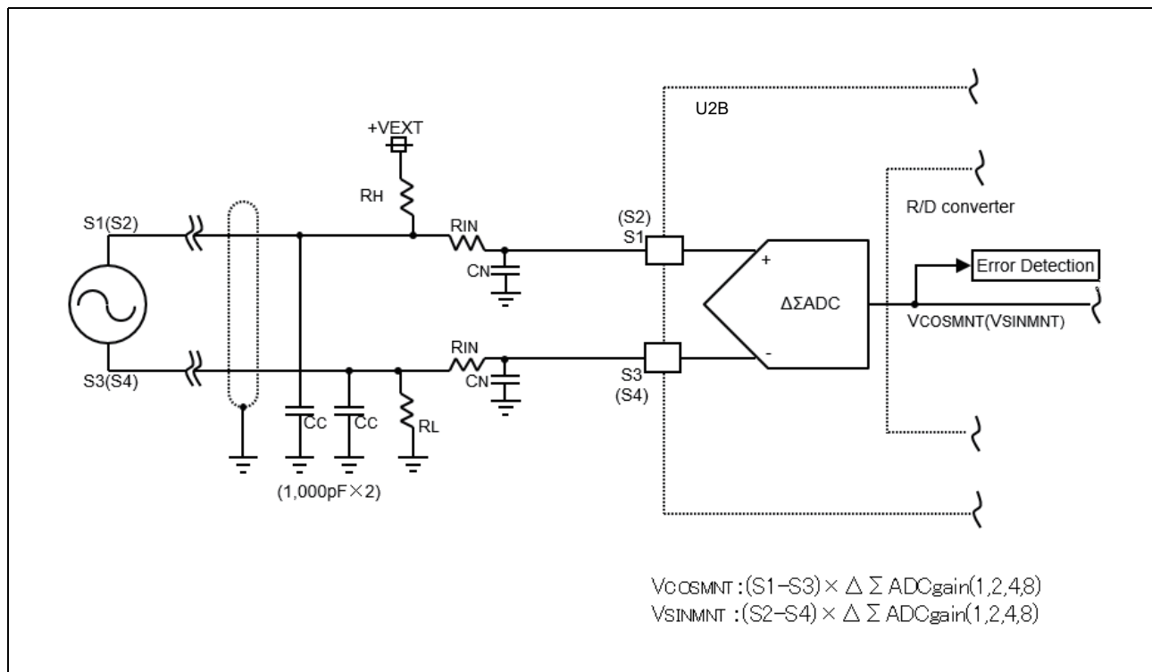
Figure 49.60 Resolver Signal Input Circuit
