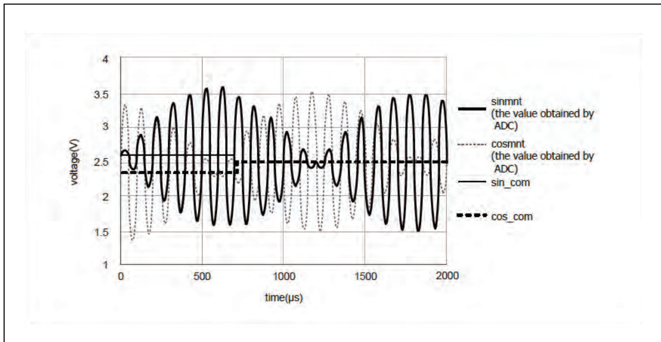
Figure 49.9 Correction of Common Offsets to 2.5V ( = 0.5 \times \text{AFCVCC} )
