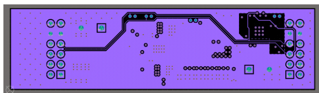
Figure 13. Layer 4 (Signal)
