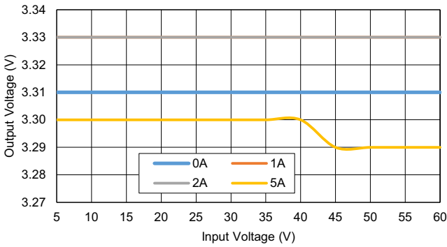
Figure 19. Line Regulation
