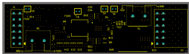
Figure 16. Bottom Overlay
