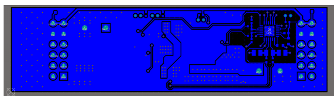
Figure 15. Bottom Layer
