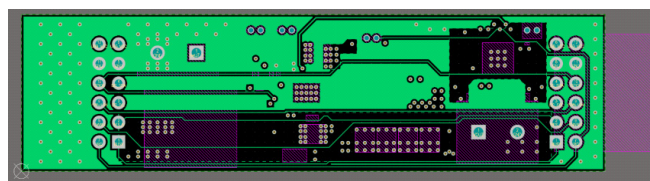
Figure 12. Layer 3 (Signal)
