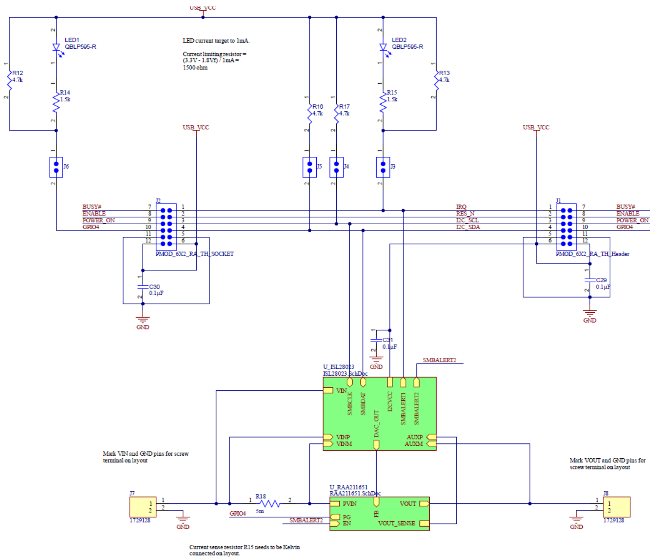
Figure 6. CIOT-5APWRPOCZ Schematic
