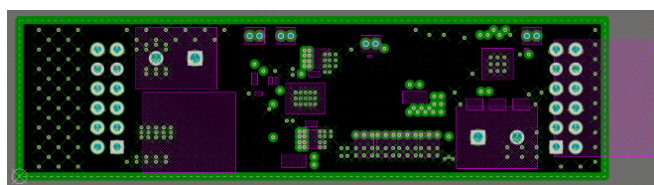
Figure 11. Layer 2 (GND)
