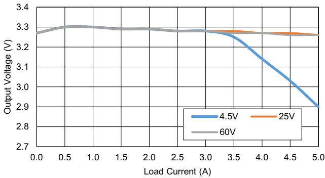
Figure 18. Load Regulation
