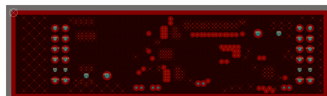
Figure 14. Layer 5 (GND)
