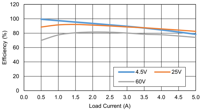
Figure 17. Efficiency
