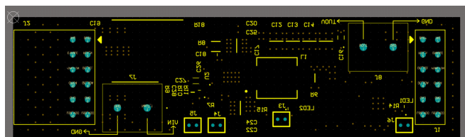
Figure 9. Top Overlay
