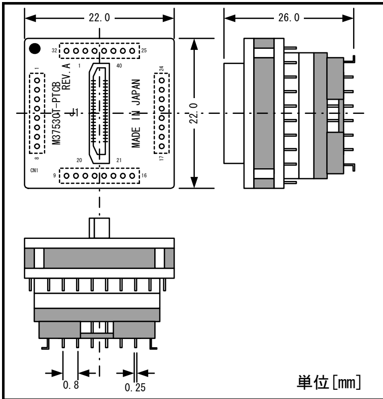
図3 M37530T-PTCB寸法図
