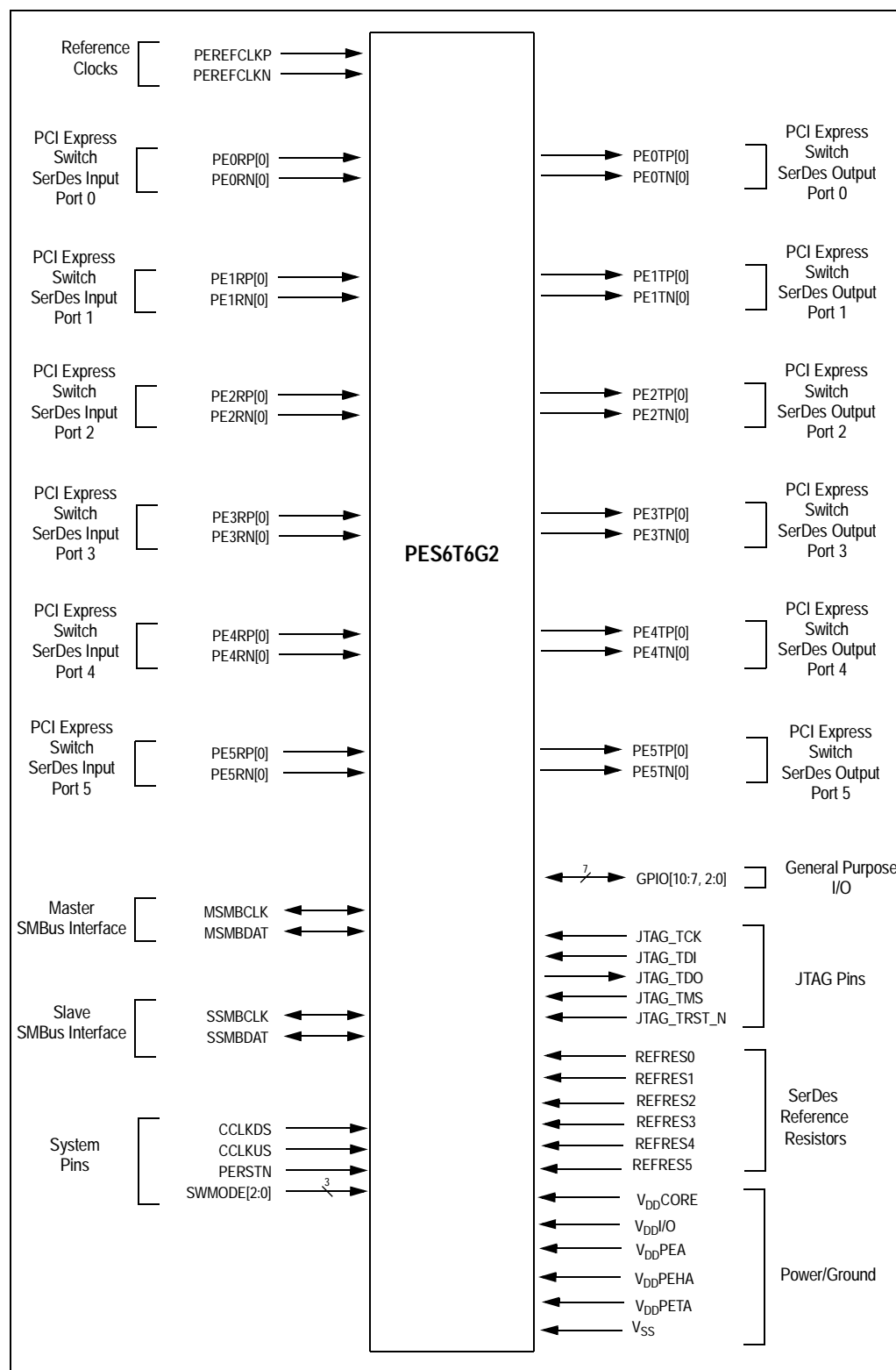
Figure 1.2 PES6T6G2 Logic Diagram
