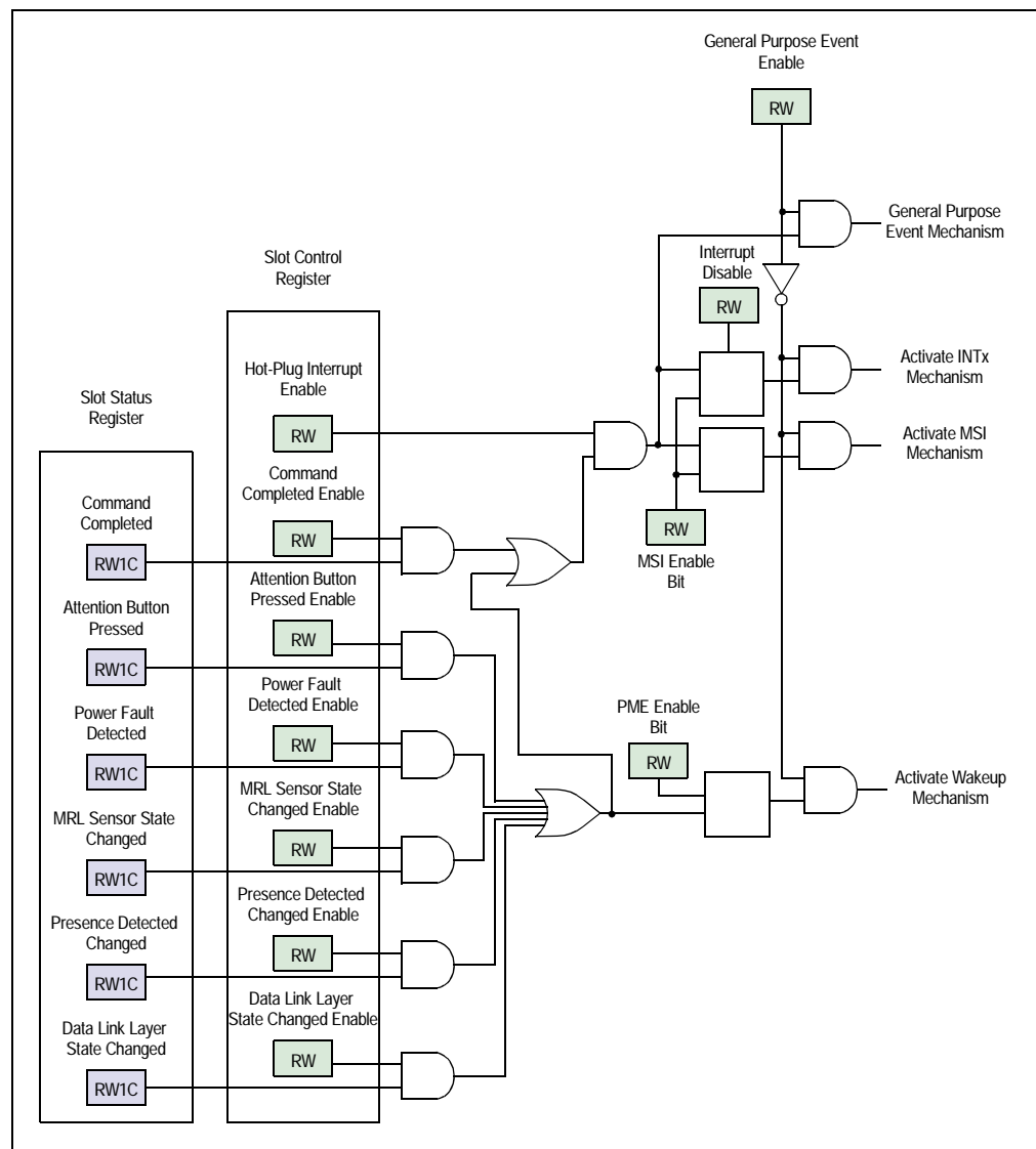
Figure 7.4 PES6T6G2 Hot-Plug Event Signalling
