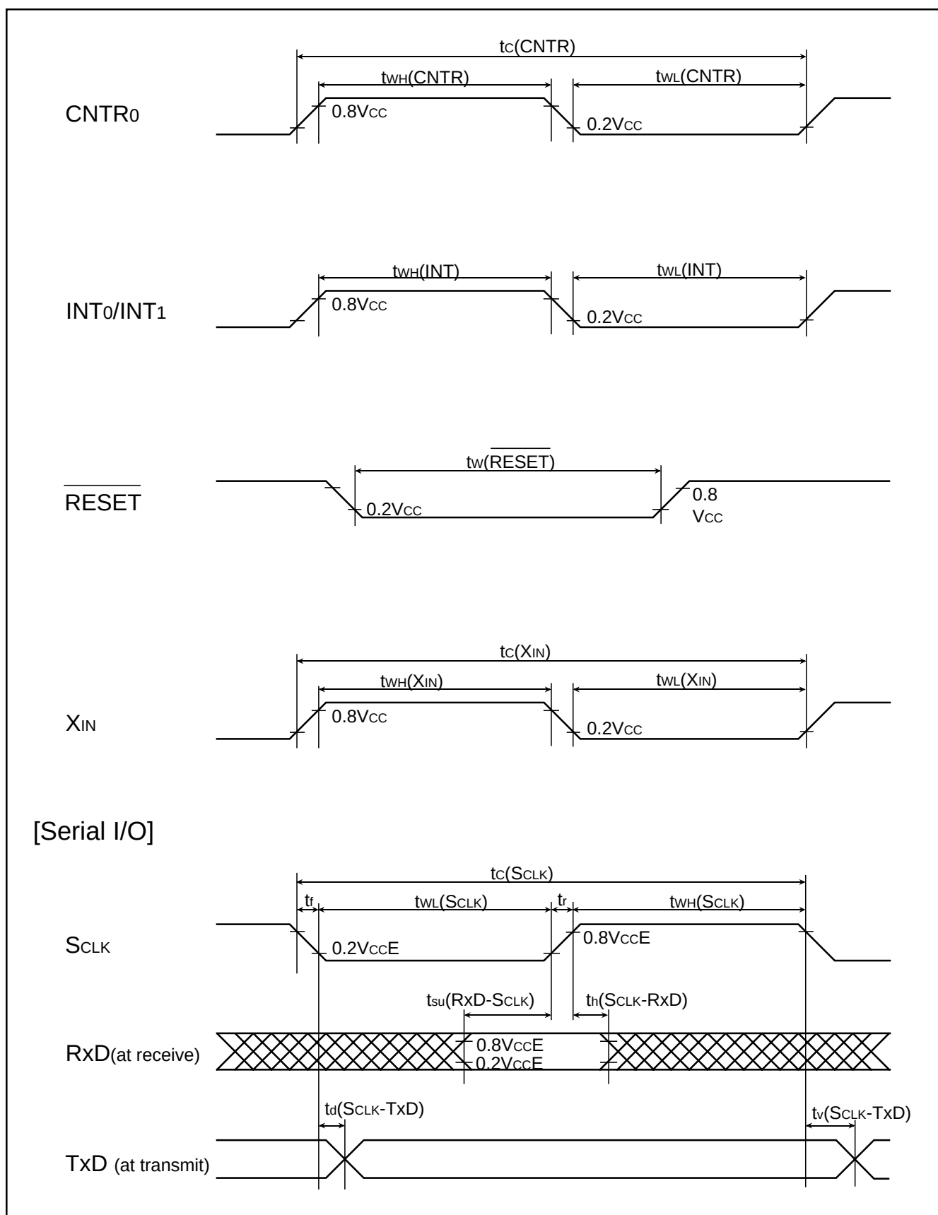
Fig. 3.1.4 Timing chart (1)
