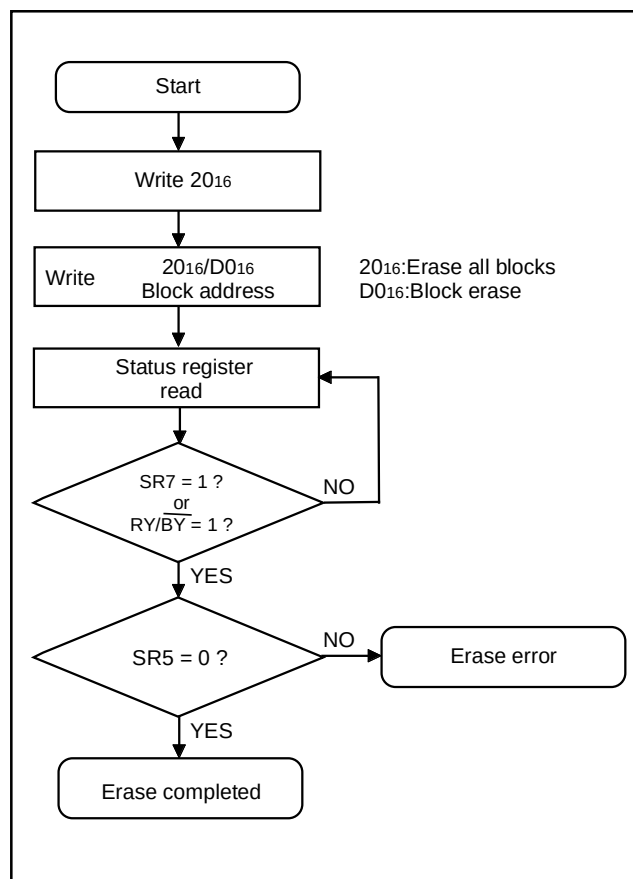
Fig. 120 Erase flowchart
