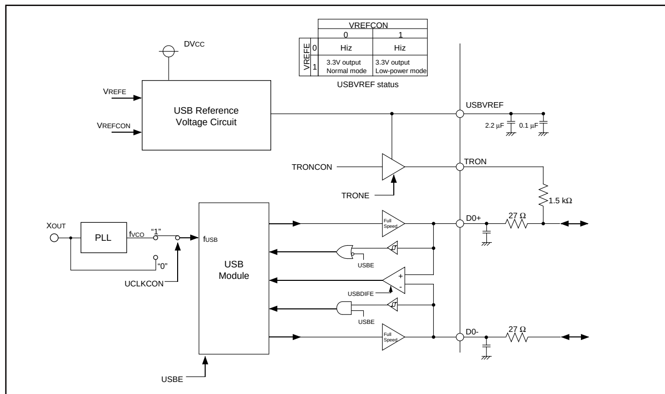
Fig. 25 USB port external circuit (D0+, D0-, USBVREF, TrON) block diagram ( 4.0V \leq V_{CC} \leq 5.25V )
