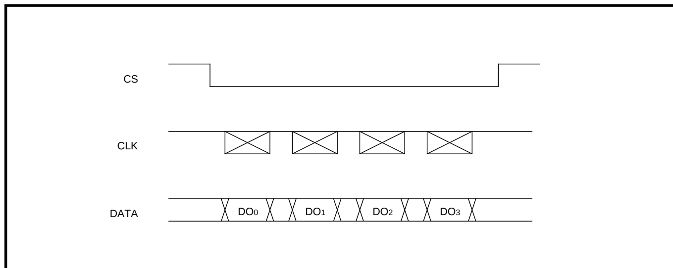
Fig. 2.4.20 Timing chart
