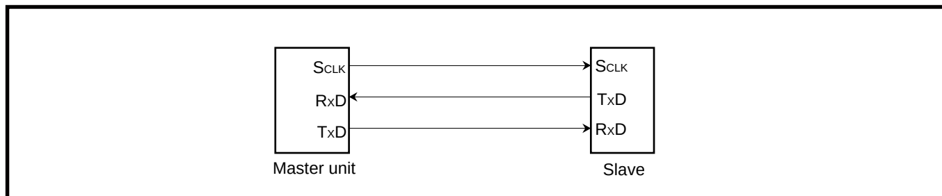
Fig. 2.4.24 Connection diagram
