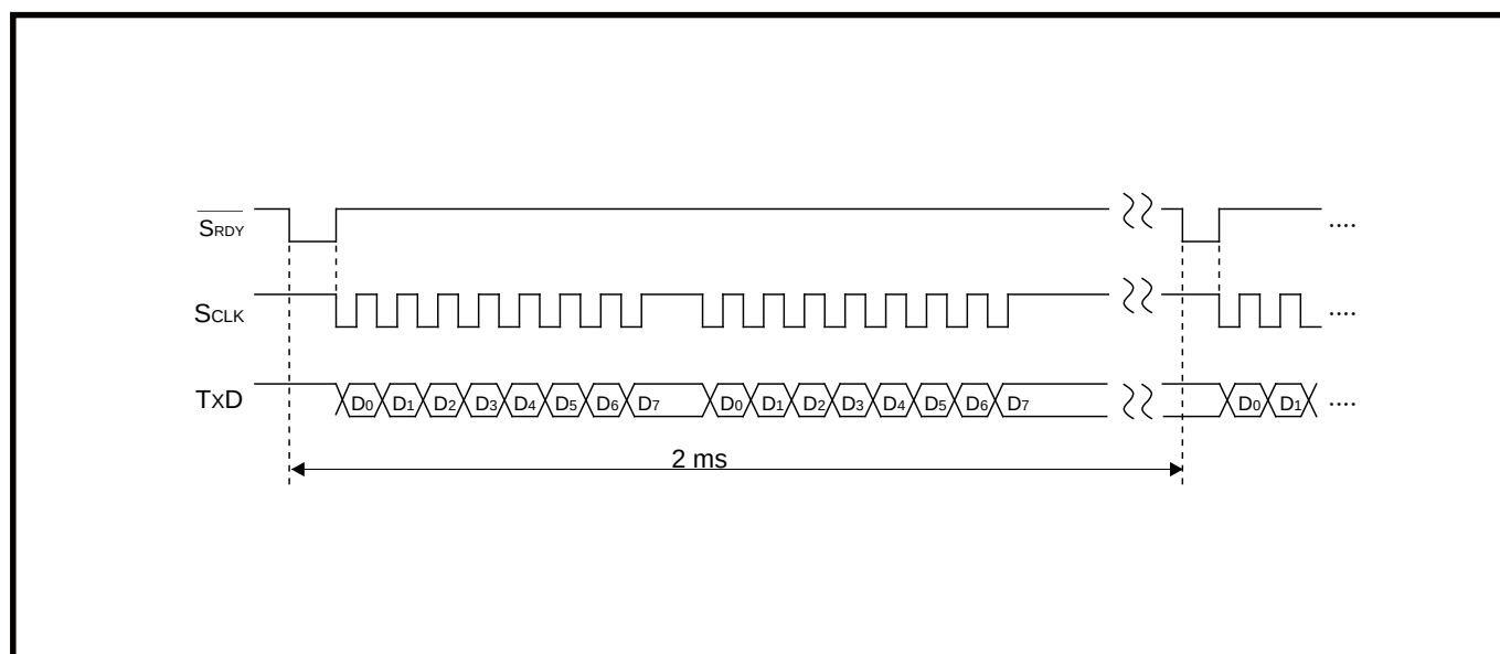
Fig. 2.4.14 Timing chart
