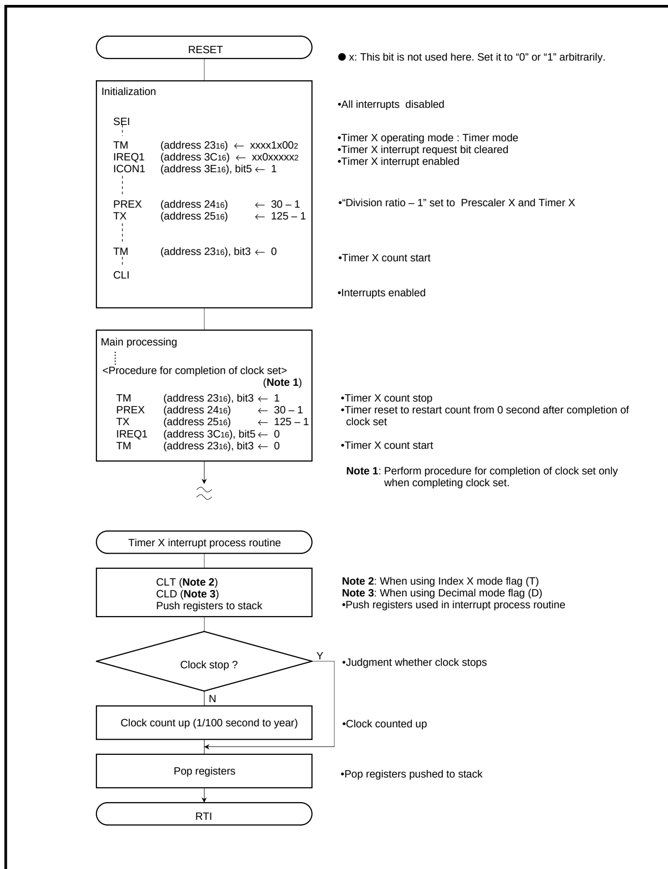
Fig. 2.3.12 Control procedure
