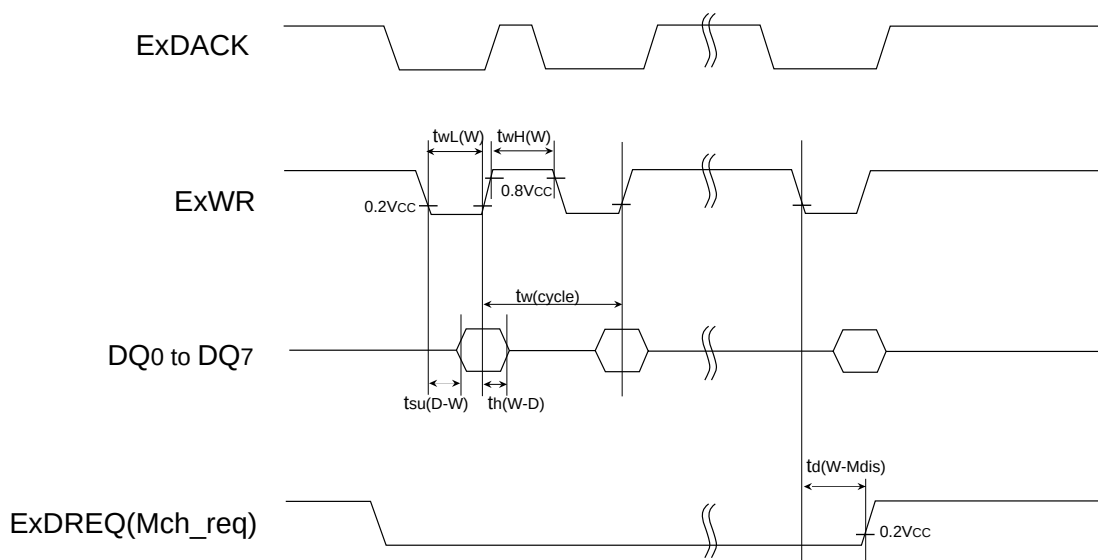
Fig. 3.1.9 Timing chart (6)
