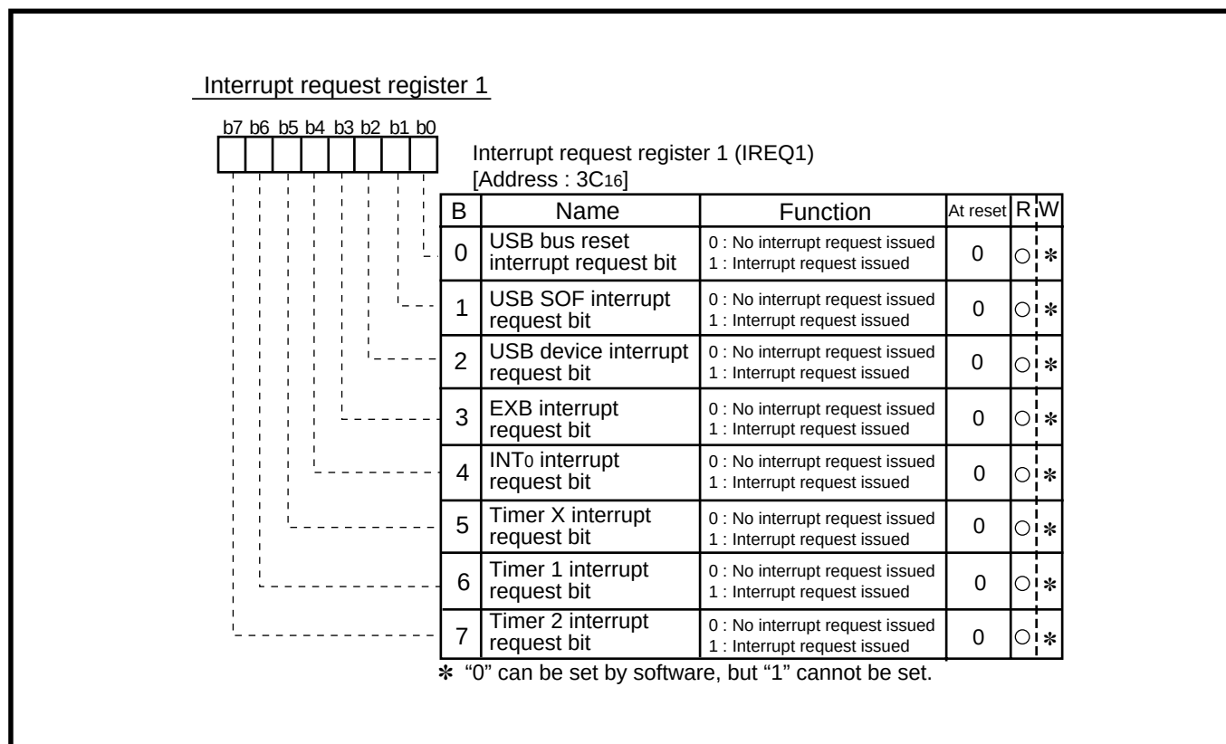
Fig. 2.2.2 Structure of Interrupt request register 1
