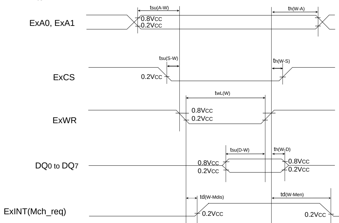
Fig. 3.1.6 Timing chart (3)
