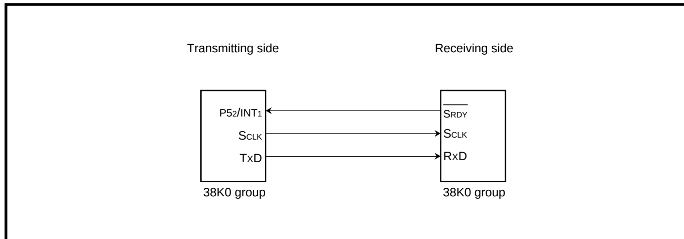
Fig. 2.4.13 Connection diagram
