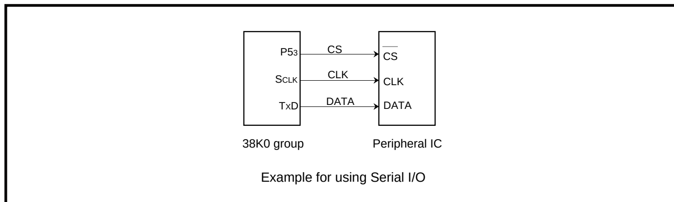
Fig. 2.4.19 Connection diagram
