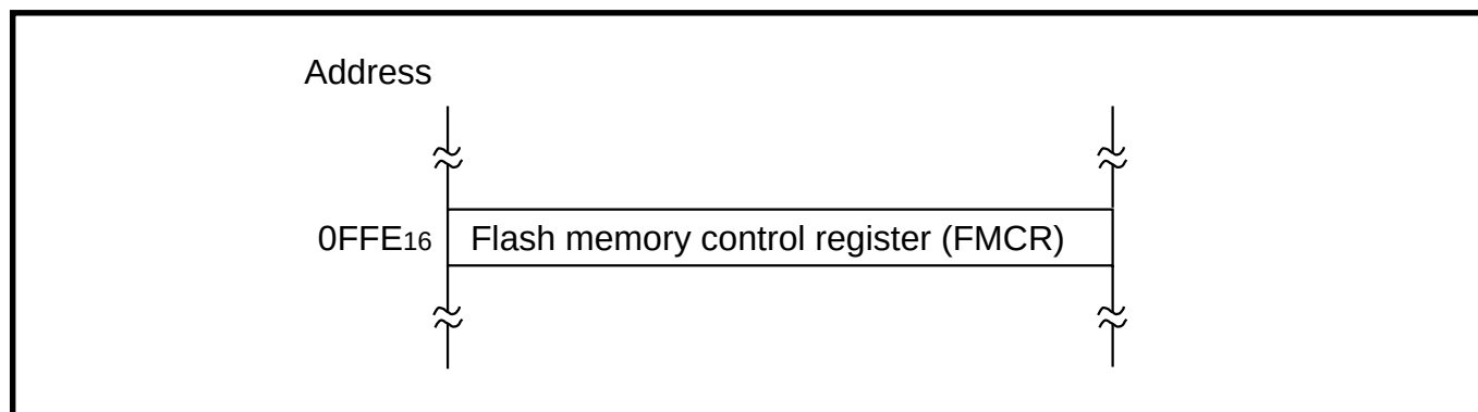
Fig. 2.13.2 Memory map of registers related to flash memory
