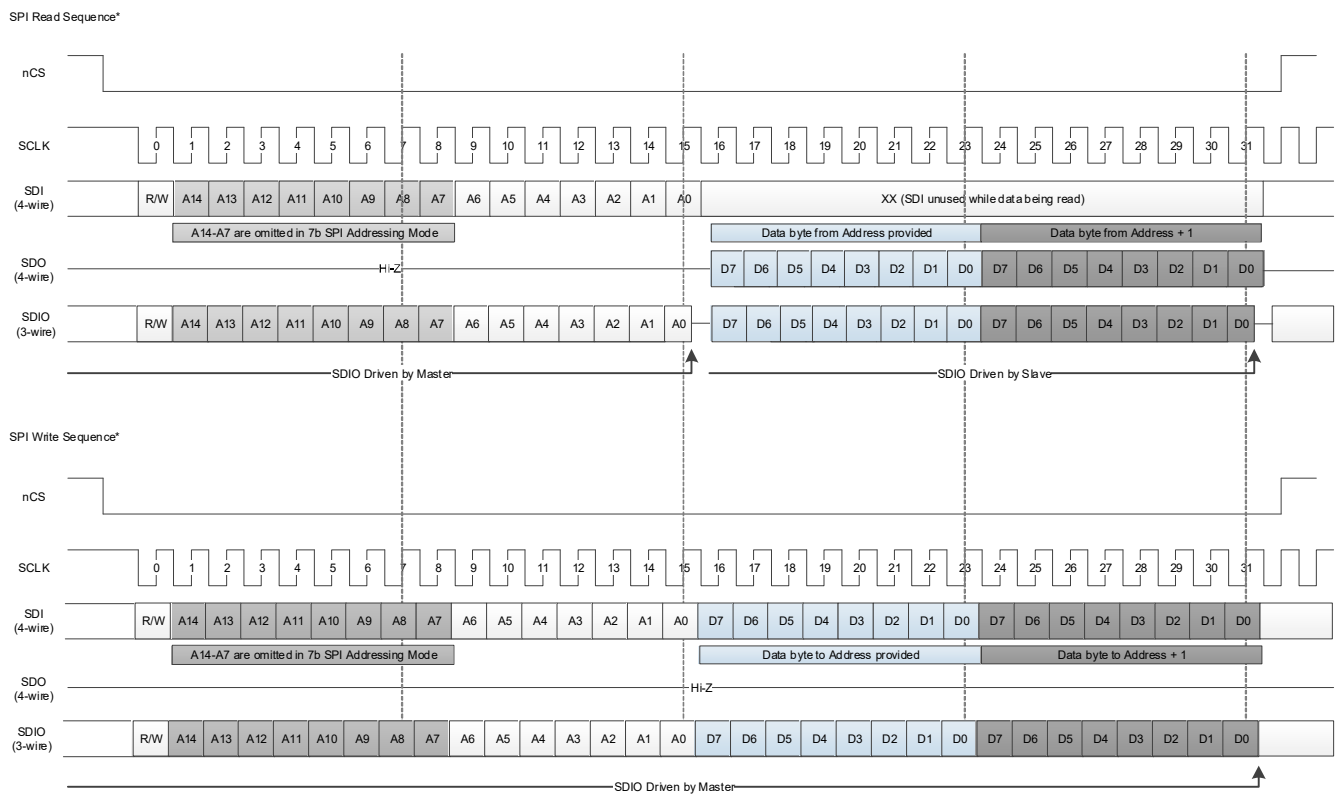
Figure 30. SPI Sequencing
