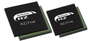
361pin LFBGA 266pin LFBGA
