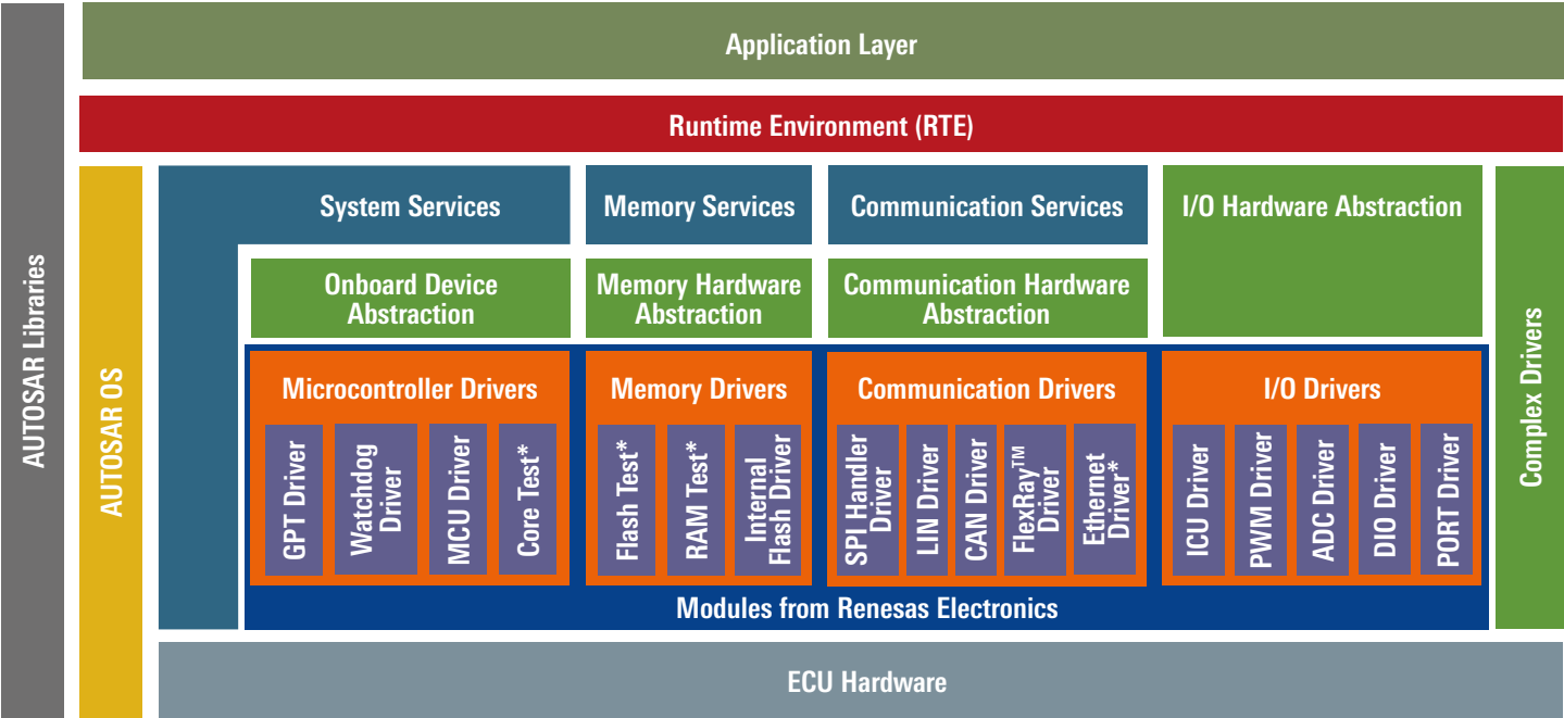
AUTOSAR basic software modules including Microcontroller Abstraction Layer (MCAL)
