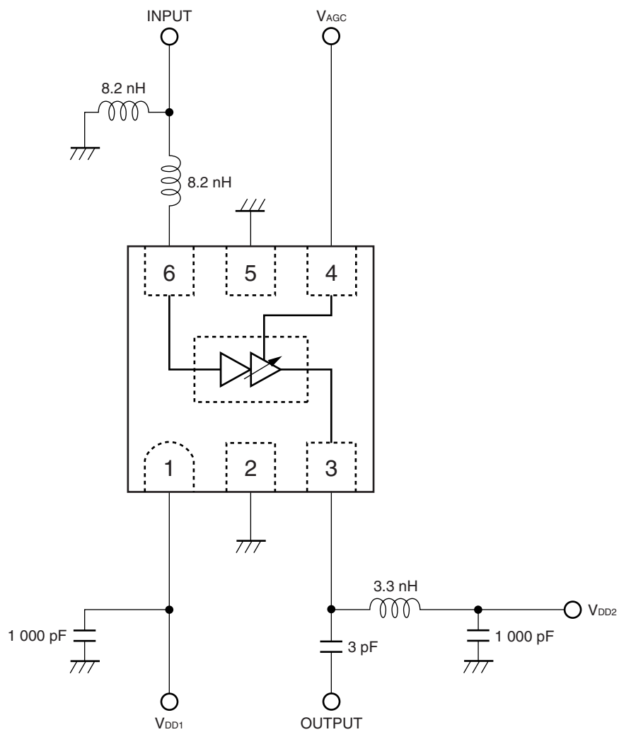
評価回路図 ( f = 1\,429 \sim 1\,453 MHz, V_{DD1} = 2.8 V, V_{DD2} = 3.2 V, V_{AGC} = 0.5 \sim 2.0 V )
