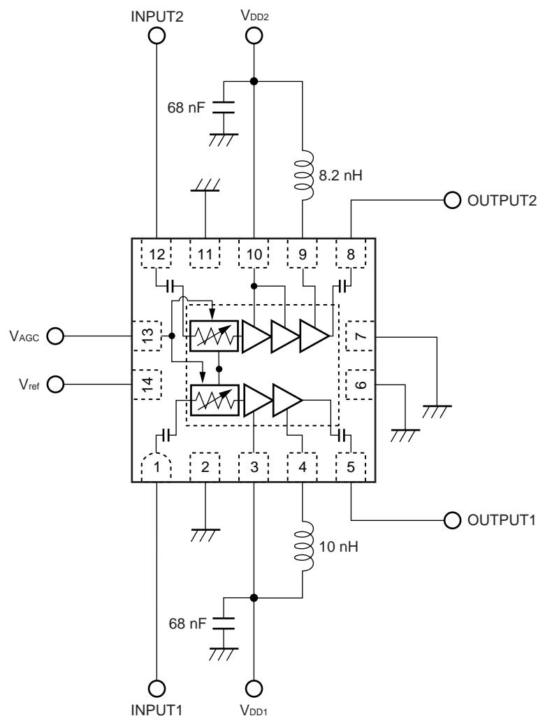
評価回路図 ( f_{opt1} = 893 \sim 960 \text{ MHz} , f_{opt2} = 1\,429 \sim 1\,468 \text{ MHz} , V_{DD1,2} = 3.2 \text{ V} )
