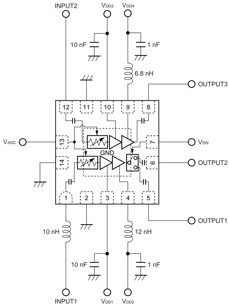
評価回路図 ( f_{opt1} = 893 \sim 960 \text{ MHz} , f_{opt2} = 1\,429 \sim 1\,453 \text{ MHz} , V_{DD1,3} = 2.8 \text{ V} , V_{DD2,4} = 3.5 \text{ V} )
