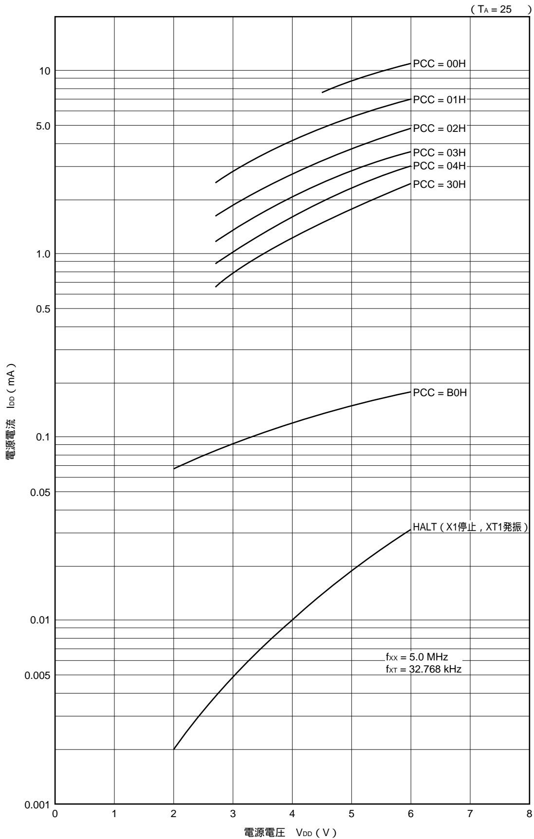
I_{DD} vs V_{DD} ( f_x = f_{xx} = 5.0 \text{ MHz} )
