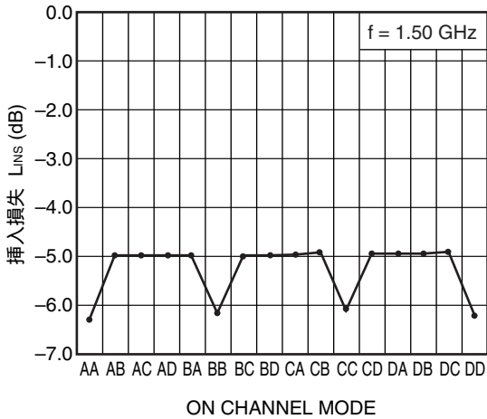
挿入損失 vs. ON CHANNEL MODE
