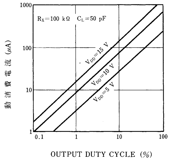
TOTAL SUPPLY CURRENT vs. OUTPUT DUTY CYCLE
