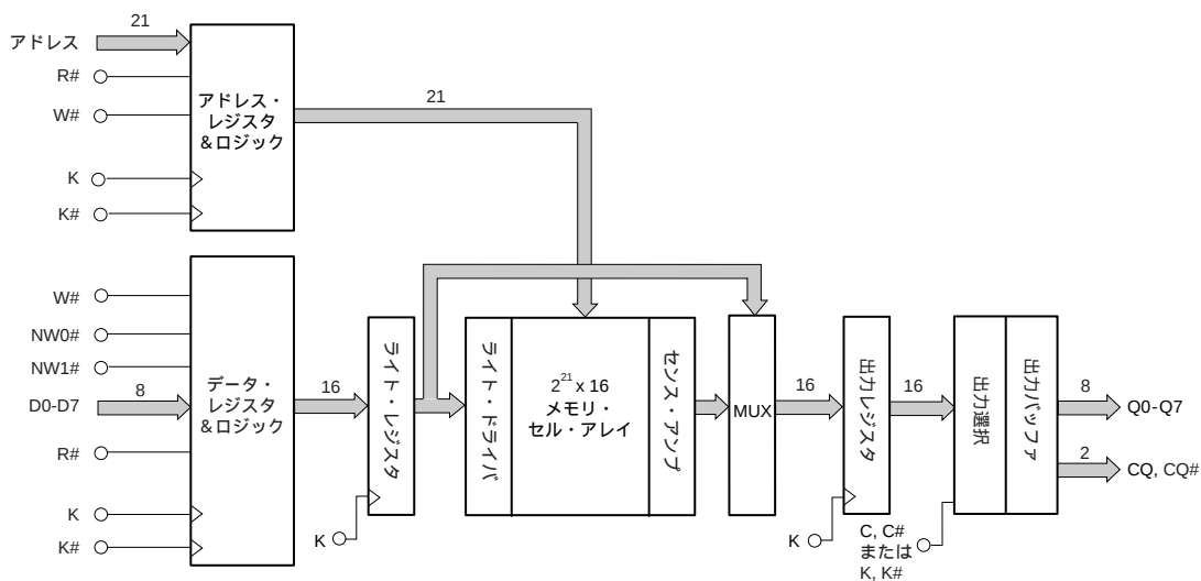
[ \mu PD44325082-A]
