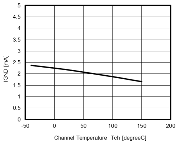
Operating current per channel VS. Channel TEMPERATURE
