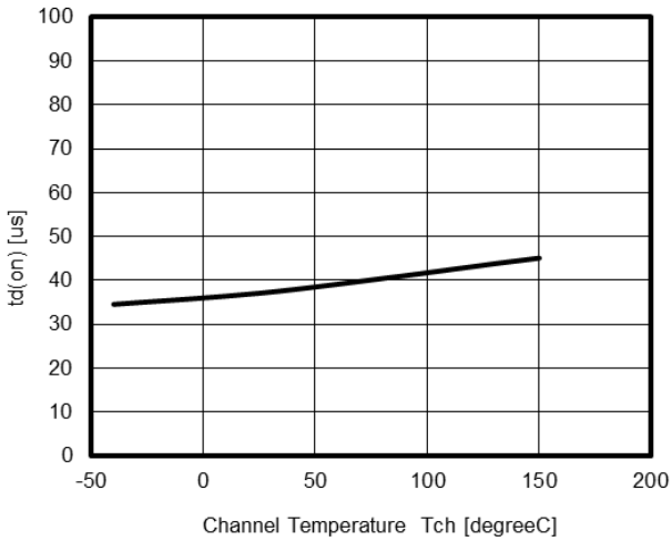
Turn on delay time VS. Channel TEMPERATURE
