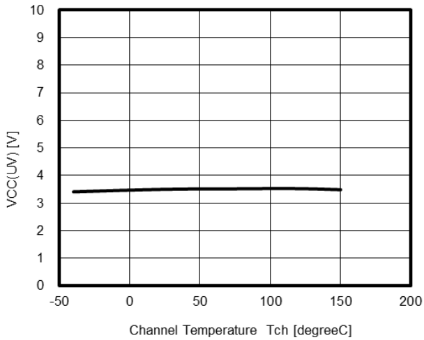
Under voltage shutdown VS. Channel TEMPERATURE
