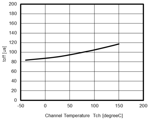
Turn off time VS. Channel TEMPERATURE
