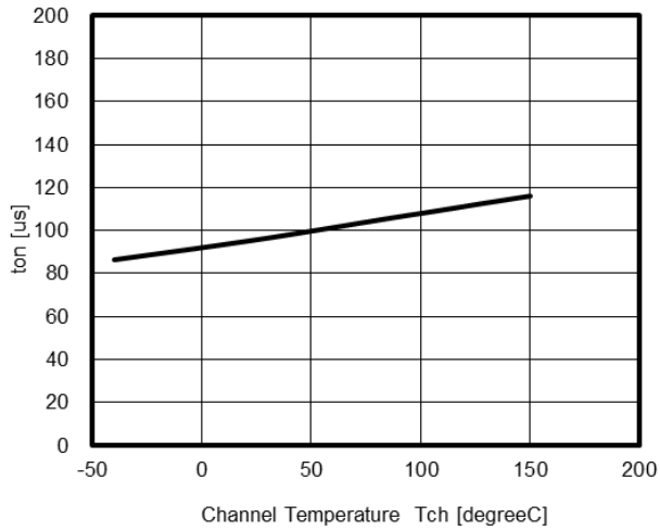
Turn on time VS. Channel TEMPERATURE
