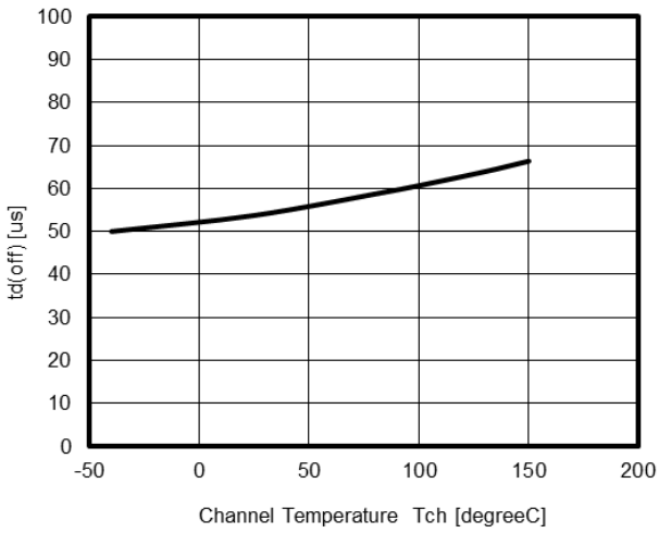
Turn off delay time VS. Channel TEMPERATURE
