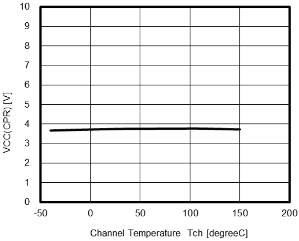
Under voltage restart VS. Channel TEMPERATURE
