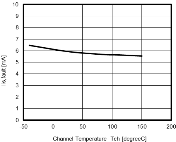
Sense current under fault condition VS. Channel TEMPERATURE
