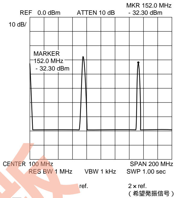
Spectrum of Overtone Oscillation.( without RF signal )
