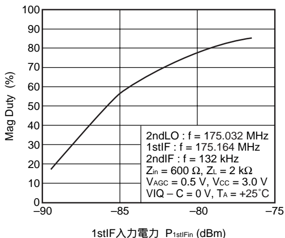
MAG DUTY vs. 1stIF入力電力
