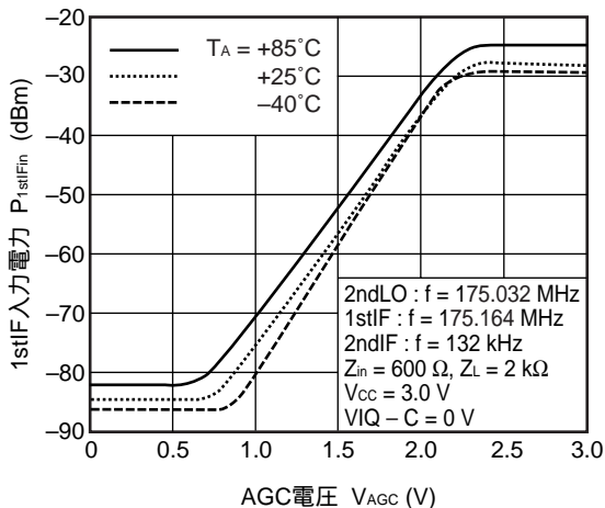
P1stIFin (MAG DUTY 50%時) vs. AGC電圧
