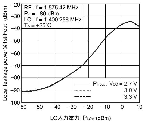
Local leakage power@1stIFout vs. LO入力電力
