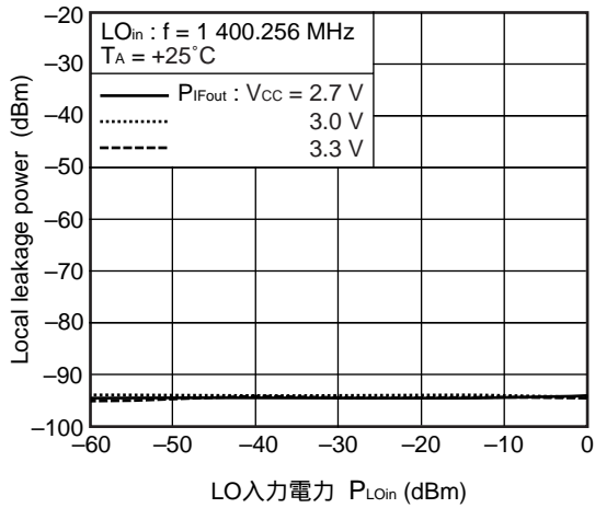
LOCAL LEAKAGE POWER vs. LO入力電力
