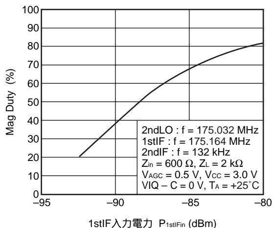
MAG DUTY vs. 1stIF入力電力
