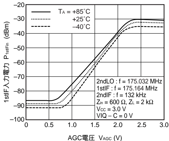
P1stIFin (MAG DUTY 50%時) vs. AGC電圧
