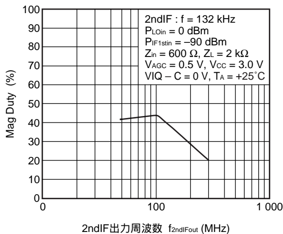
MAG DUTY vs. 2ndIF出力周波数
