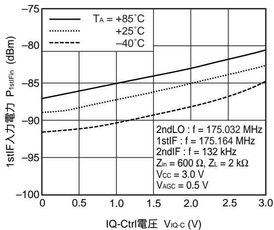
P1stIFin (MAG DUTY 50%時) vs. IQ Ctrl電圧
