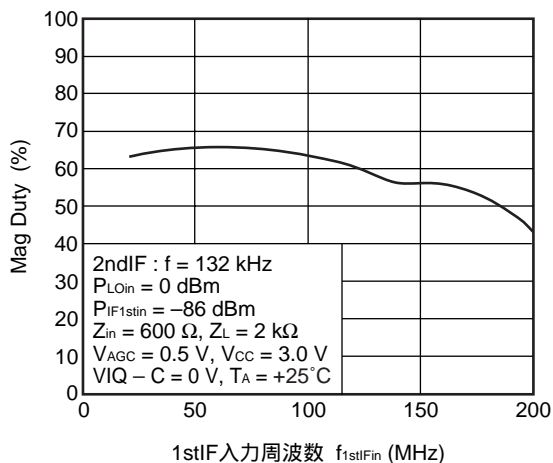
MAG DUTY vs. 1stIF入力周波数
