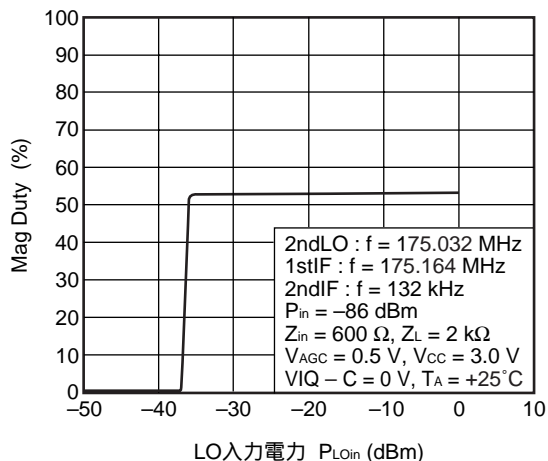
MAG DUTY vs. LO入力電力
