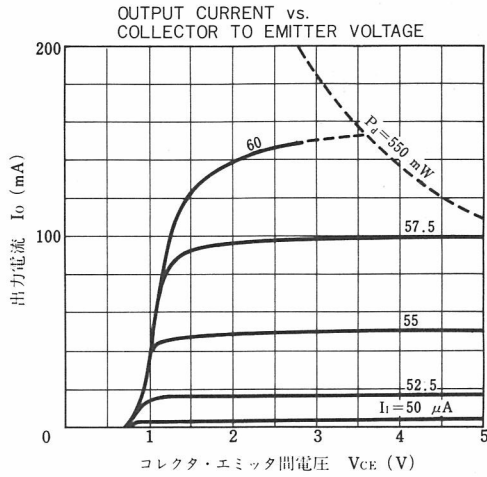
特性曲線/TYPICAL CHARACTERISTICS( T_a=25^\circ\text{C} )
