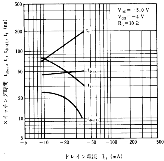
SWITCHING CHARACTERISTICS
