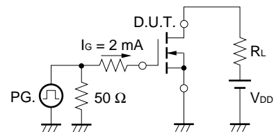
TEST CIRCUIT 3 GATE CHARGE
