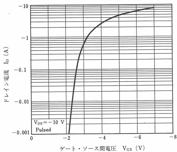
TRANSFER CHARACTERISTIC
